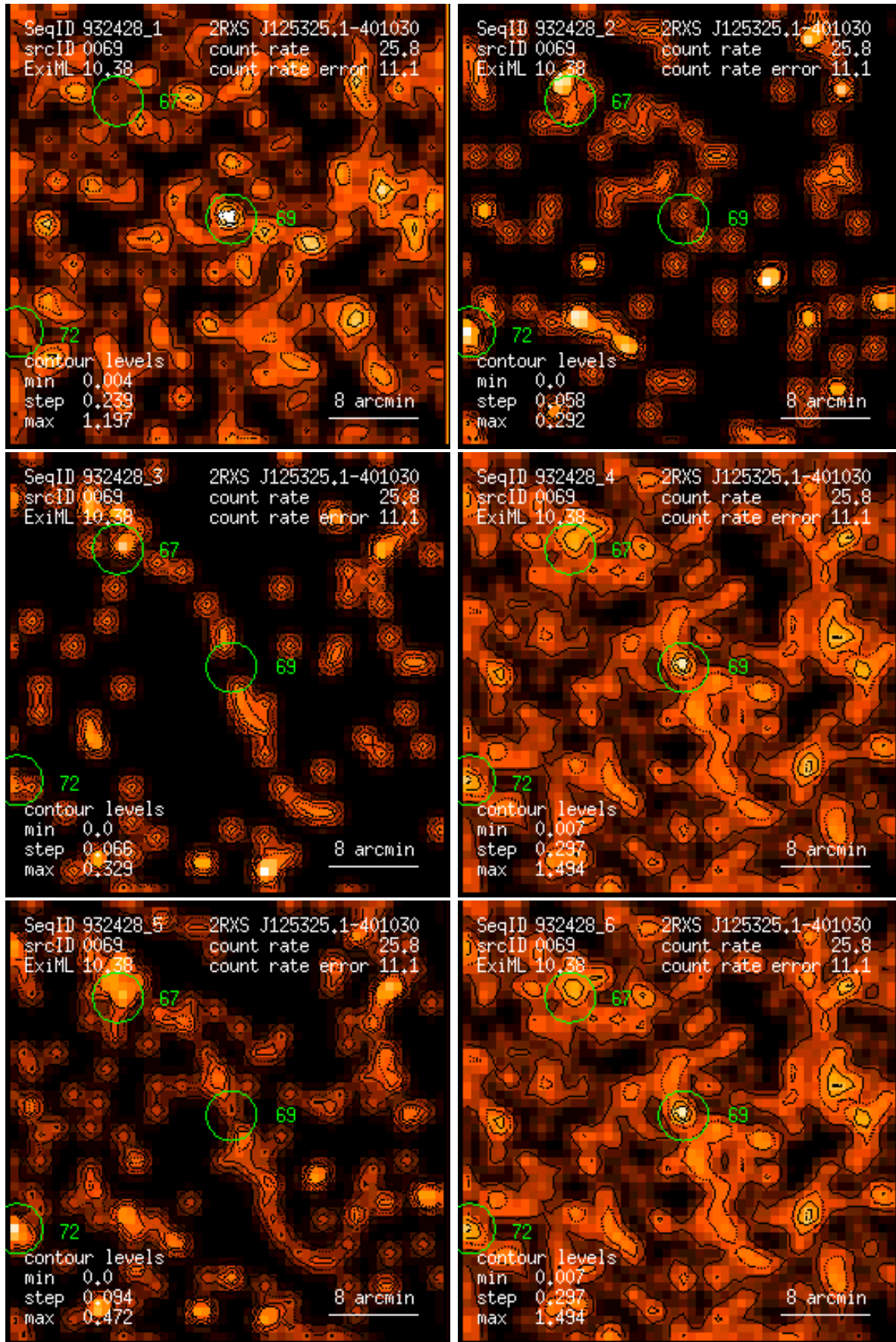
Figure 69: RASS 932428: detection 0069: band rate images, Gaussian filter: (1) PSPC channels 11 – 41, (2) 52 – 90, (3) 91 – 201, (4) 11 – 235, (5) 52 – 201, (6) 11 – 201. Broad band rates in counts/ks. Band rate contour levels in counts/ks/arcmin 2 .
