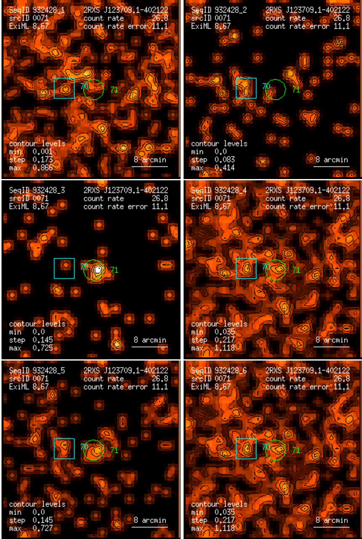
Figure 71: RASS 932428: detection 0071: band rate images, Gaussian filter: (1) PSPC channels 11 – 41, (2) 52 – 90, (3) 91 – 201, (4) 11 – 235, (5) 52 – 201, (6) 11 – 201. Broad band rates in counts/ks. Band rate contour levels in counts/ks/arcmin 2 .
