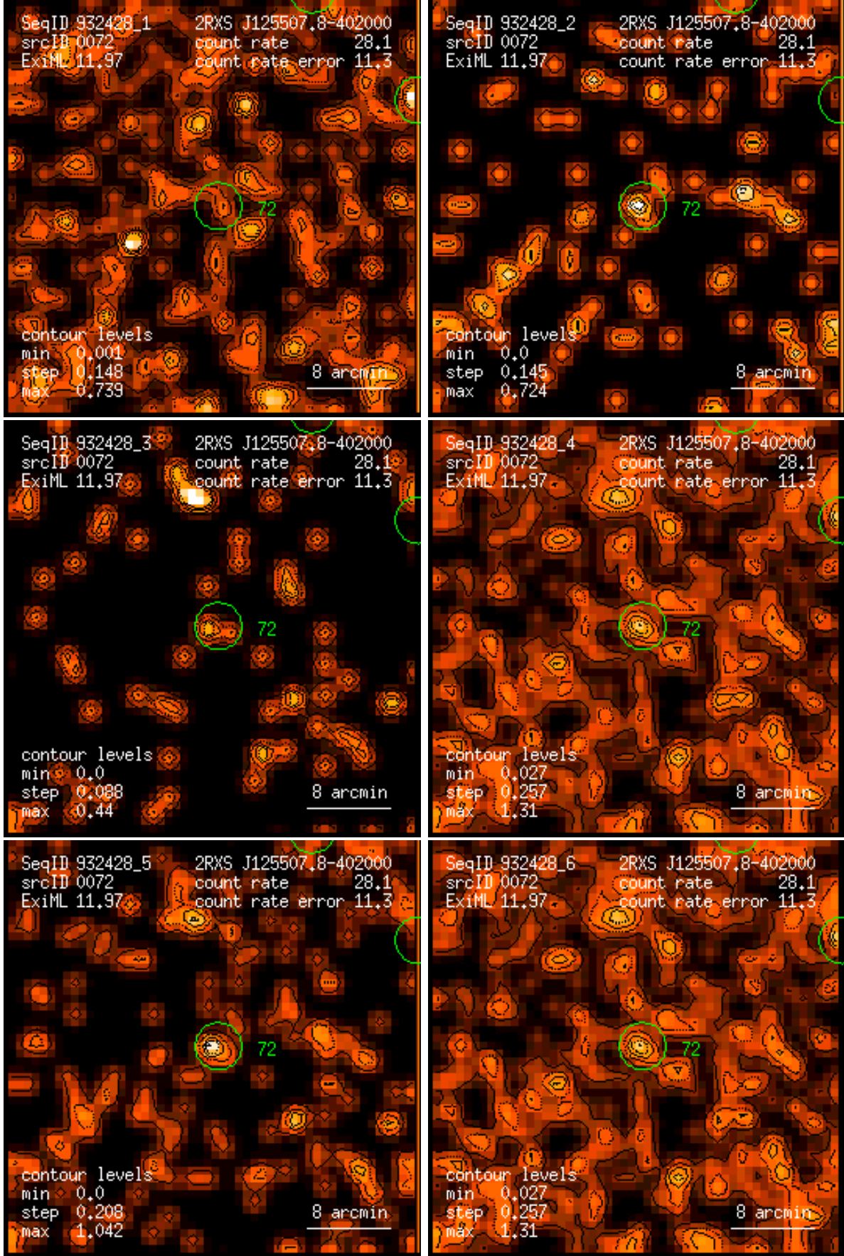
Figure 72: RASS 932428: detection 0072: band rate images, Gaussian filter: (1) PSPC channels 11 – 41, (2) 52 – 90, (3) 91 – 201, (4) 11 – 235, (5) 52 – 201, (6) 11 – 201. Broad band rates in counts/ks. Band rate contour levels in counts/ks/arcmin 2 .
