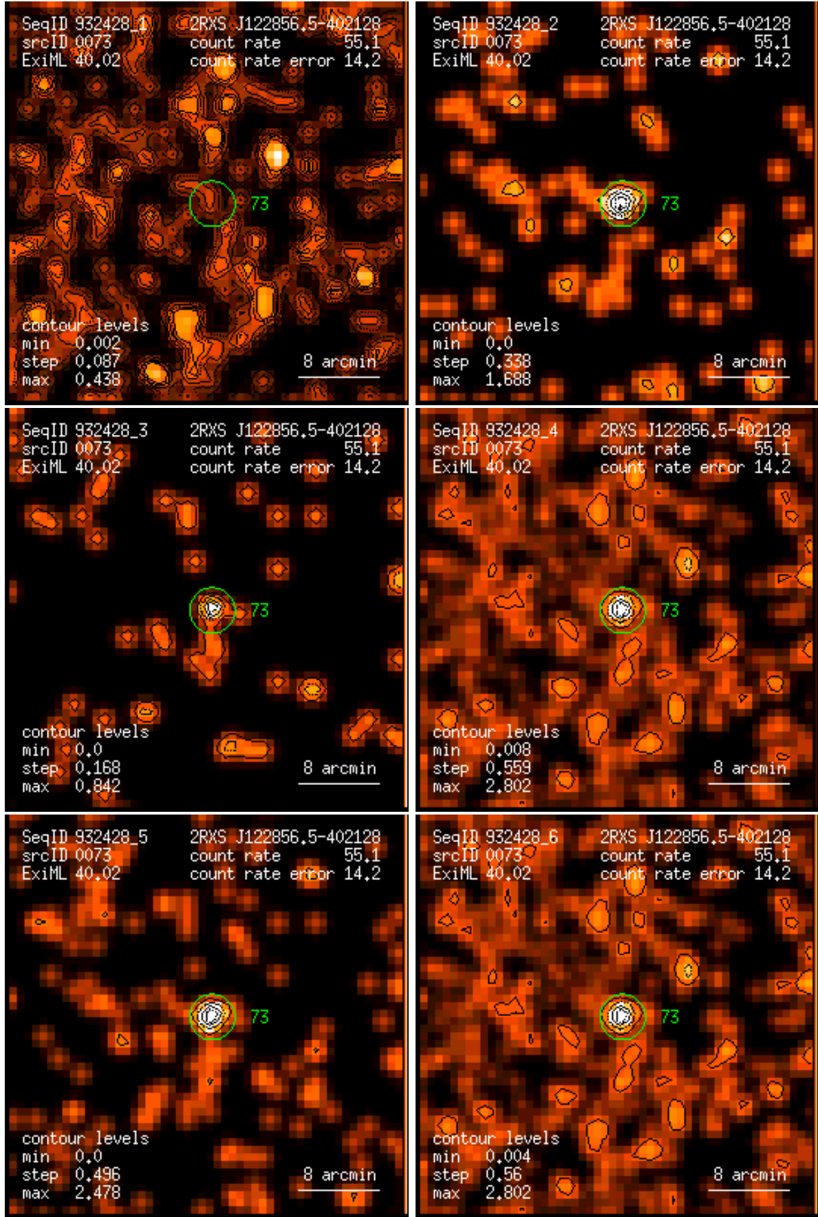
Figure 73: RASS 932428: detection 0073: band rate images, Gaussian filter: (1) PSPC channels 11 – 41, (2) 52 – 90, (3) 91 – 201, (4) 11 – 235, (5) 52 – 201, (6) 11 – 201. Broad band rates in counts/ks. Band rate contour levels in counts/ks/arcmin 2 .
