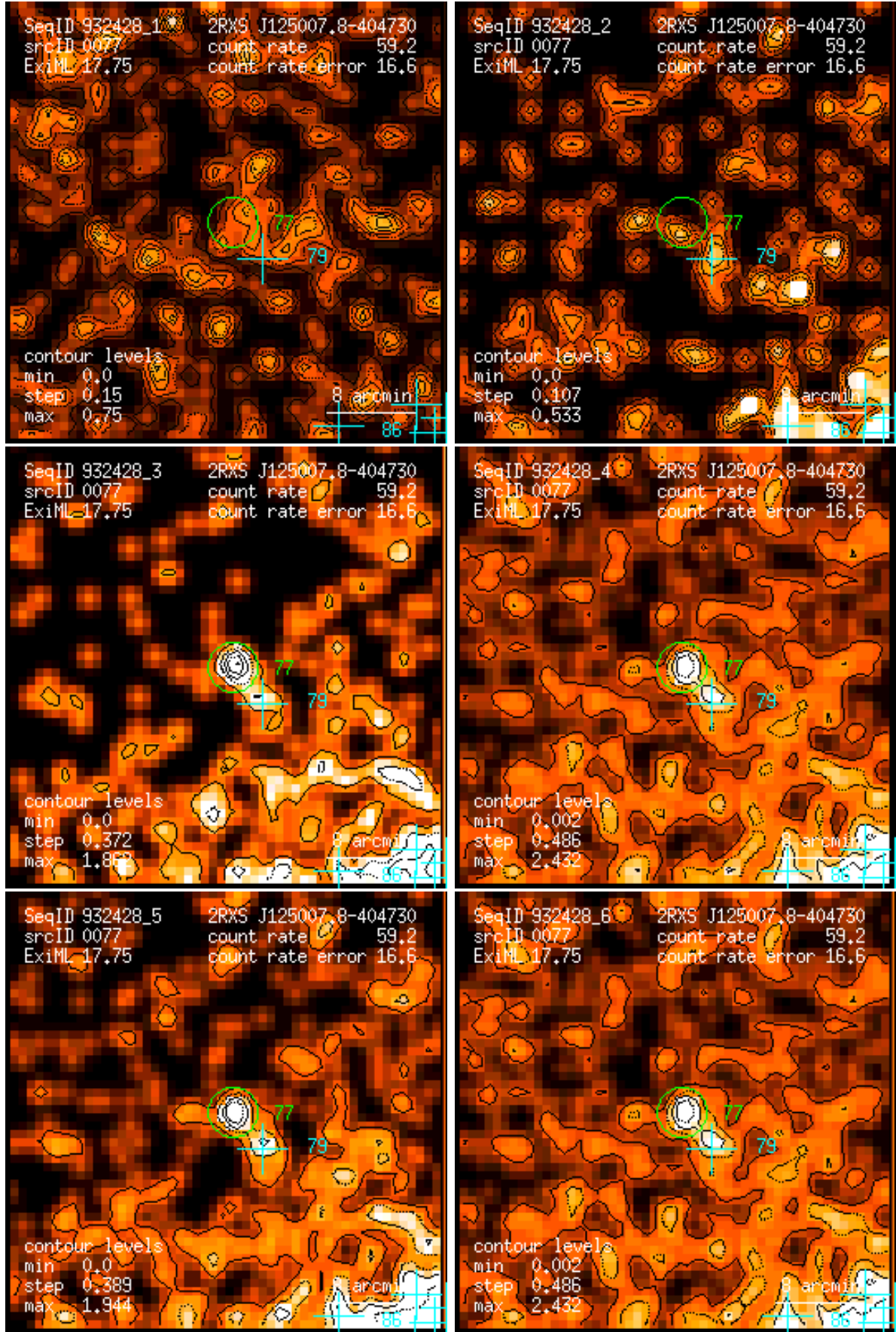
Figure 77: RASS 932428: detection 0077: band rate images, Gaussian filter: (1) PSPC channels 11 – 41, (2) 52 – 90, (3) 91 – 201, (4) 11 – 235, (5) 52 – 201, (6) 11 – 201. Broad band rates in counts/ks. Band rate contour levels in counts/ks/arcmin 2 .
