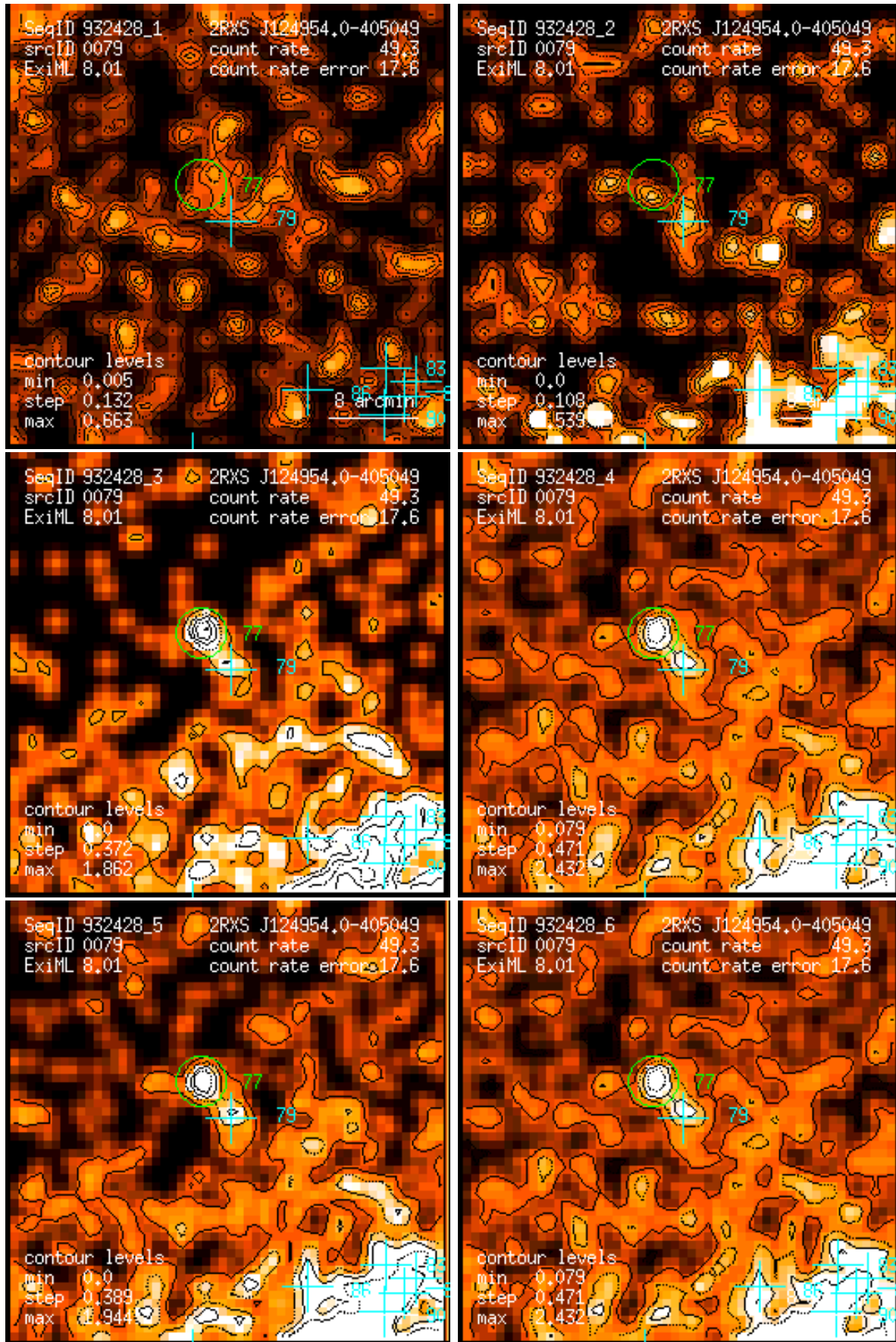
Figure 79: RASS 932428: detection 0079: band rate images, Gaussian filter: (1) PSPC channels 11 – 41, (2) 52 – 90, (3) 91 – 201, (4) 11 – 235, (5) 52 – 201, (6) 11 – 201. Broad band rates in counts/ks. Band rate contour levels in counts/ks/arcmin 2 .
