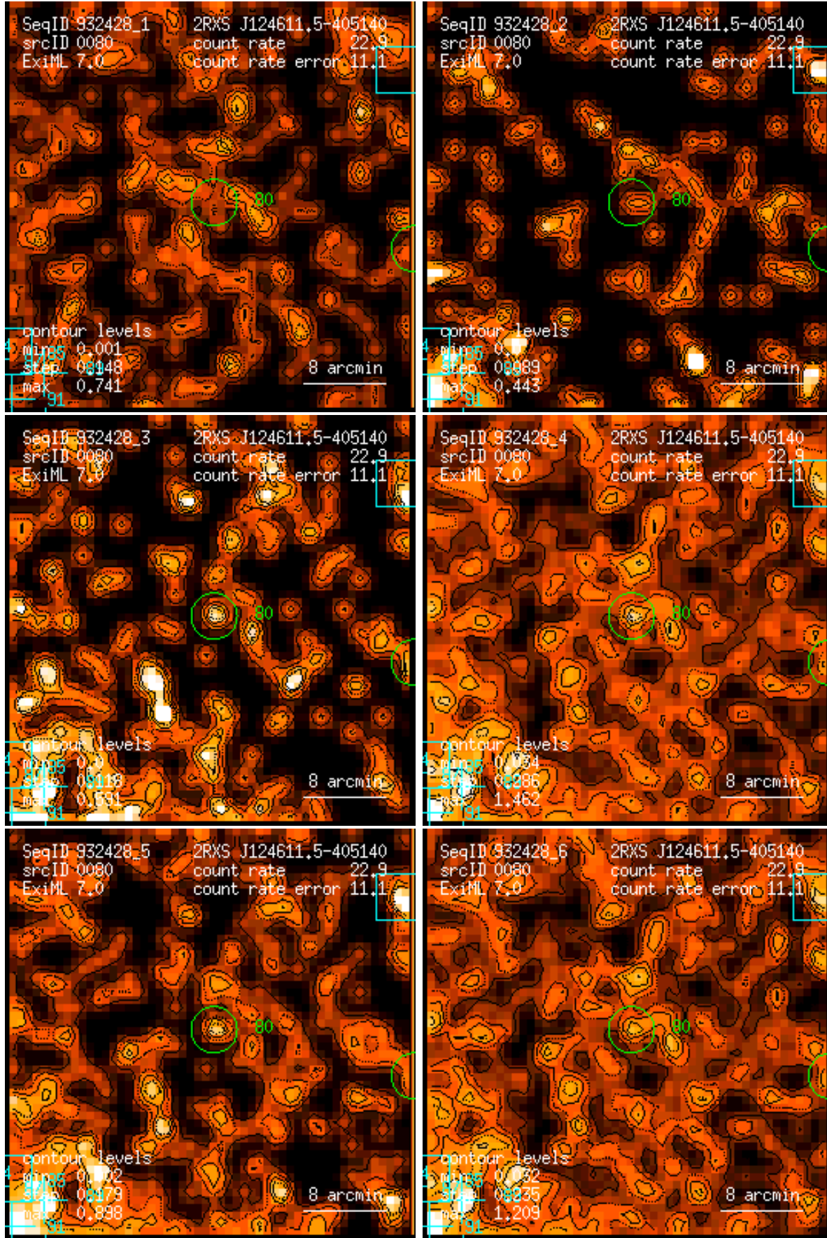
Figure 80: RASS 932428: detection 0080: band rate images, Gaussian filter: (1) PSPC channels 11 – 41, (2) 52 – 90, (3) 91 – 201, (4) 11 – 235, (5) 52 – 201, (6) 11 – 201. Broad band rates in counts/ks. Band rate contour levels in counts/ks/arcmin 2 .
