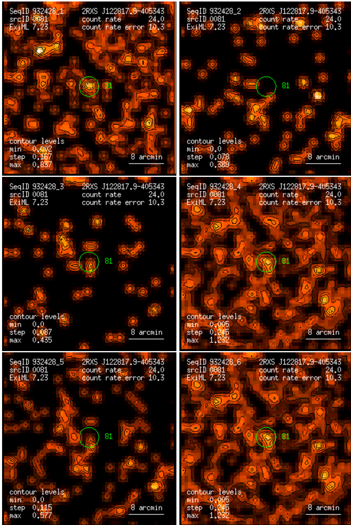
Figure 81: RASS 932428: detection 0081: band rate images, Gaussian filter: (1) PSPC channels 11 – 41, (2) 52 – 90, (3) 91 – 201, (4) 11 – 235, (5) 52 – 201, (6) 11 – 201. Broad band rates in counts/ks. Band rate contour levels in counts/ks/arcmin 2 .
