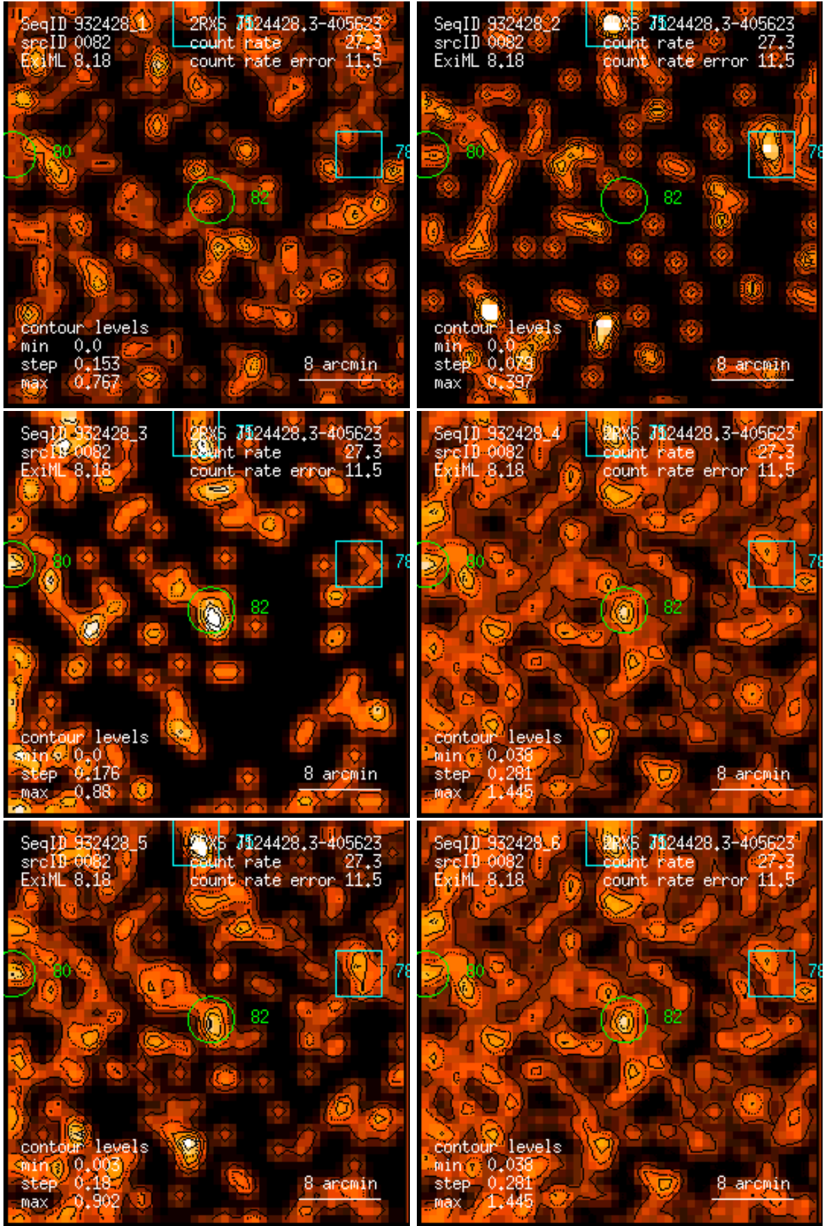
Figure 82: RASS 932428: detection 0082: band rate images, Gaussian filter: (1) PSPC channels 11 – 41, (2) 52 – 90, (3) 91 – 201, (4) 11 – 235, (5) 52 – 201, (6) 11 – 201. Broad band rates in counts/ks. Band rate contour levels in counts/ks/arcmin 2 .
