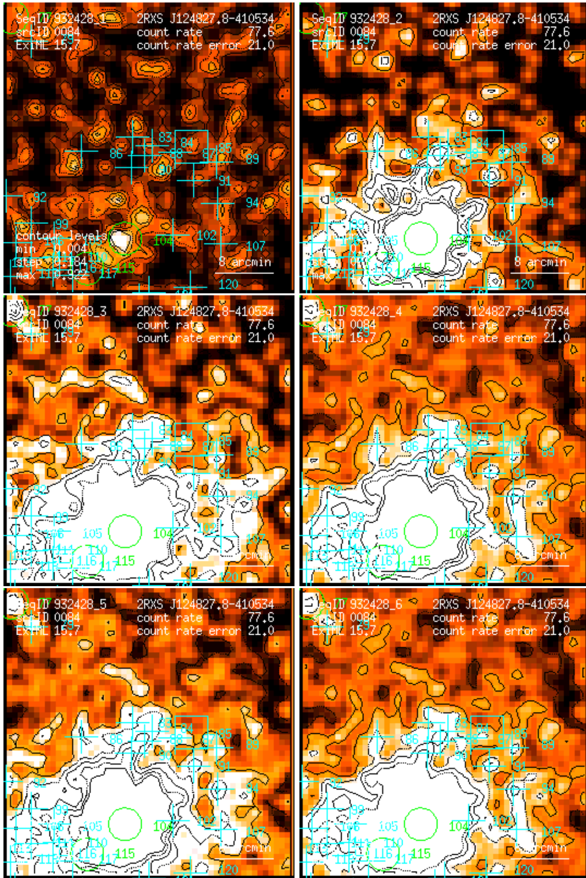
Figure 84: RASS 932428: detection 0084: band rate images, Gaussian filter: (1) PSPC channels 11 – 41, (2) 52 – 90, (3) 91 – 201, (4) 11 – 235, (5) 52 – 201, (6) 11 – 201. Broad band rates in counts/ks. Band rate contour levels in counts/ks/arcmin 2 .
