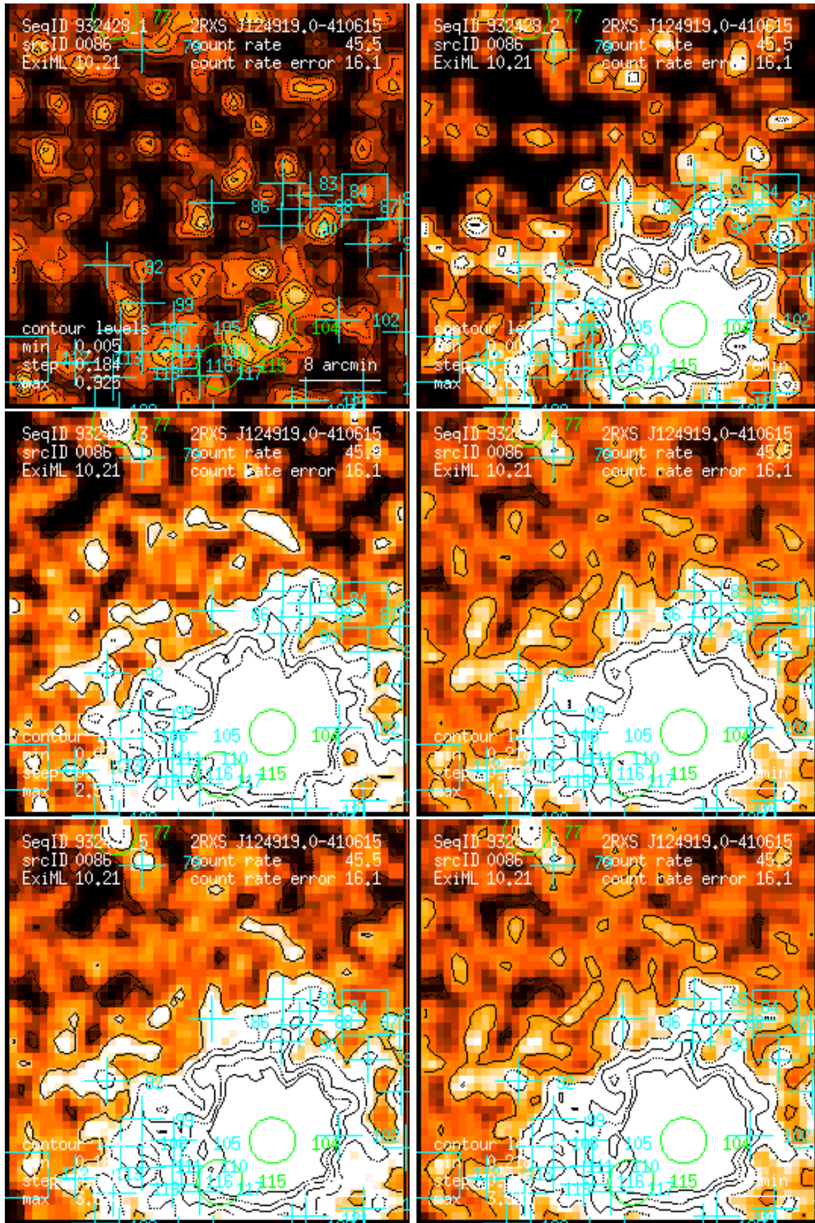
Figure 86: RASS 932428: detection 0086: band rate images, Gaussian filter: (1) PSPC channels 11 – 41, (2) 52 – 90, (3) 91 – 201, (4) 11 – 235, (5) 52 – 201, (6) 11 – 201. Broad band rates in counts/ks. Band rate contour levels in counts/ks/arcmin 2 .
