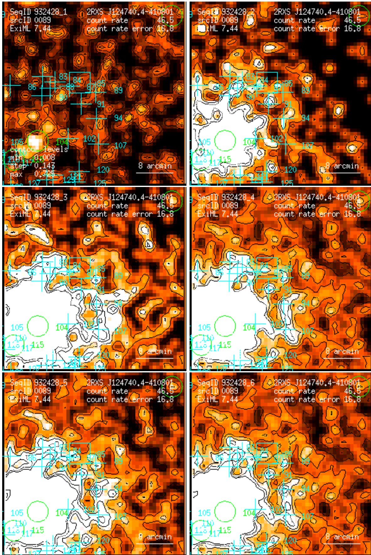
Figure 89: RASS 932428: detection 0089: band rate images, Gaussian filter: (1) PSPC channels 11 – 41, (2) 52 – 90, (3) 91 – 201, (4) 11 – 235, (5) 52 – 201, (6) 11 – 201. Broad band rates in counts/ks. Band rate contour levels in counts/ks/arcmin 2 .
