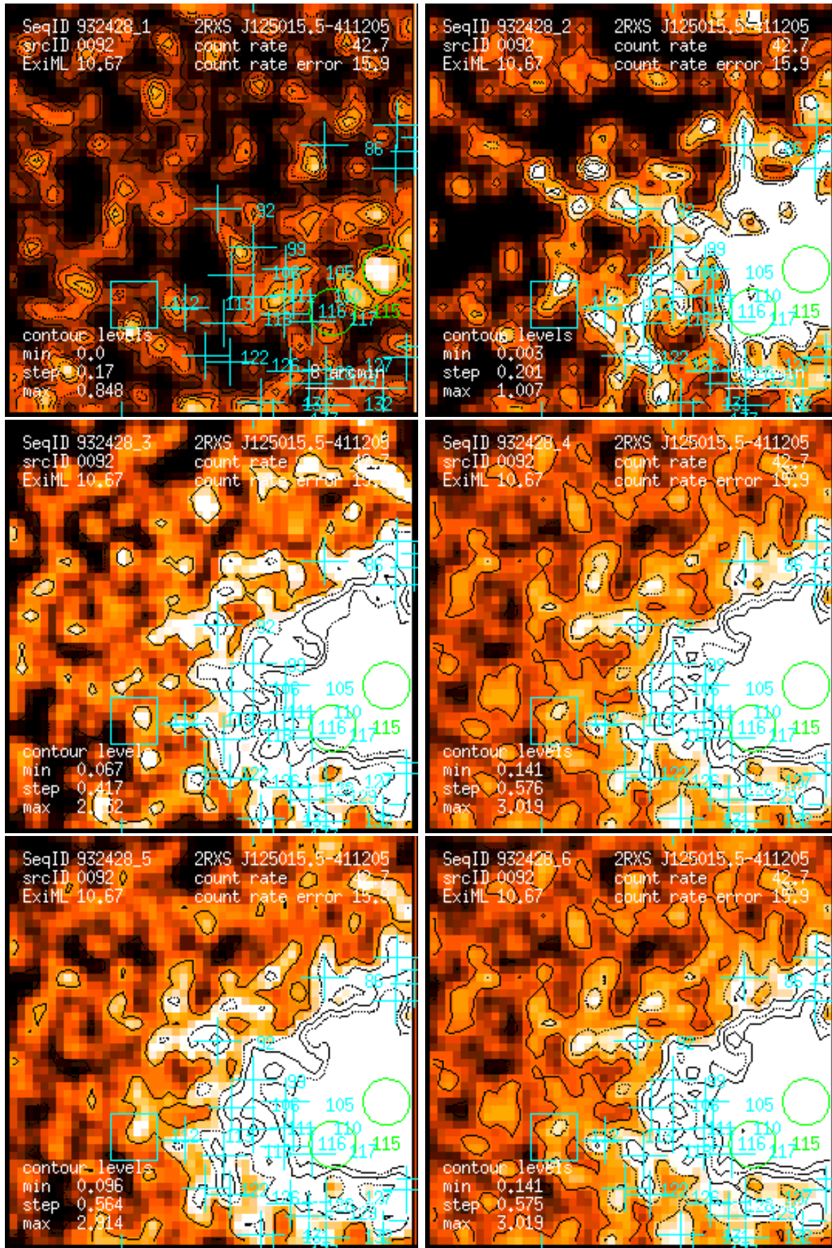
Figure 92: RASS 932428: detection 0092: band rate images, Gaussian filter: (1) PSPC channels 11 – 41, (2) 52 – 90, (3) 91 – 201, (4) 11 – 235, (5) 52 – 201, (6) 11 – 201. Broad band rates in counts/ks. Band rate contour levels in counts/ks/arcmin 2 .
