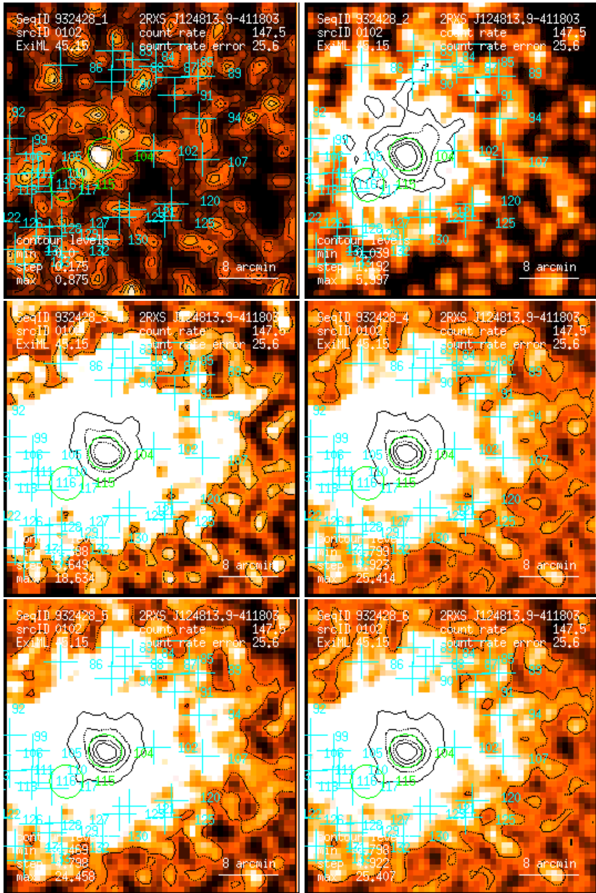
Figure 102: RASS 932428: detection 0102: band rate images, Gaussian filter: (1) PSPC channels 11 – 41, (2) 52 – 90, (3) 91 – 201, (4) 11 – 235, (5) 52 – 201, (6) 11 – 201. Broad band rates in counts/ks. Band rate contour levels in counts/ks/arcmin 2 .
