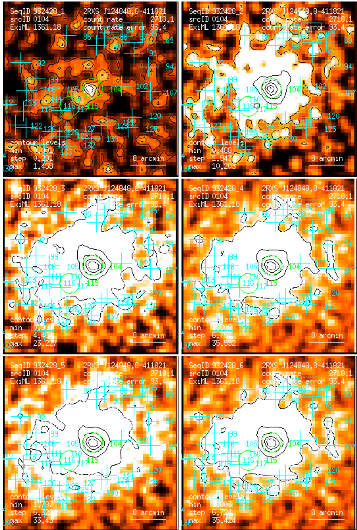
Figure 104: RASS 932428: detection 0104: band rate images, Gaussian filter: (1) PSPC channels 11 – 41, (2) 52 – 90, (3) 91 – 201, (4) 11 – 235, (5) 52 – 201, (6) 11 – 201. Broad band rates in counts/ks. Band rate contour levels in counts/ks/arcmin 2 .
