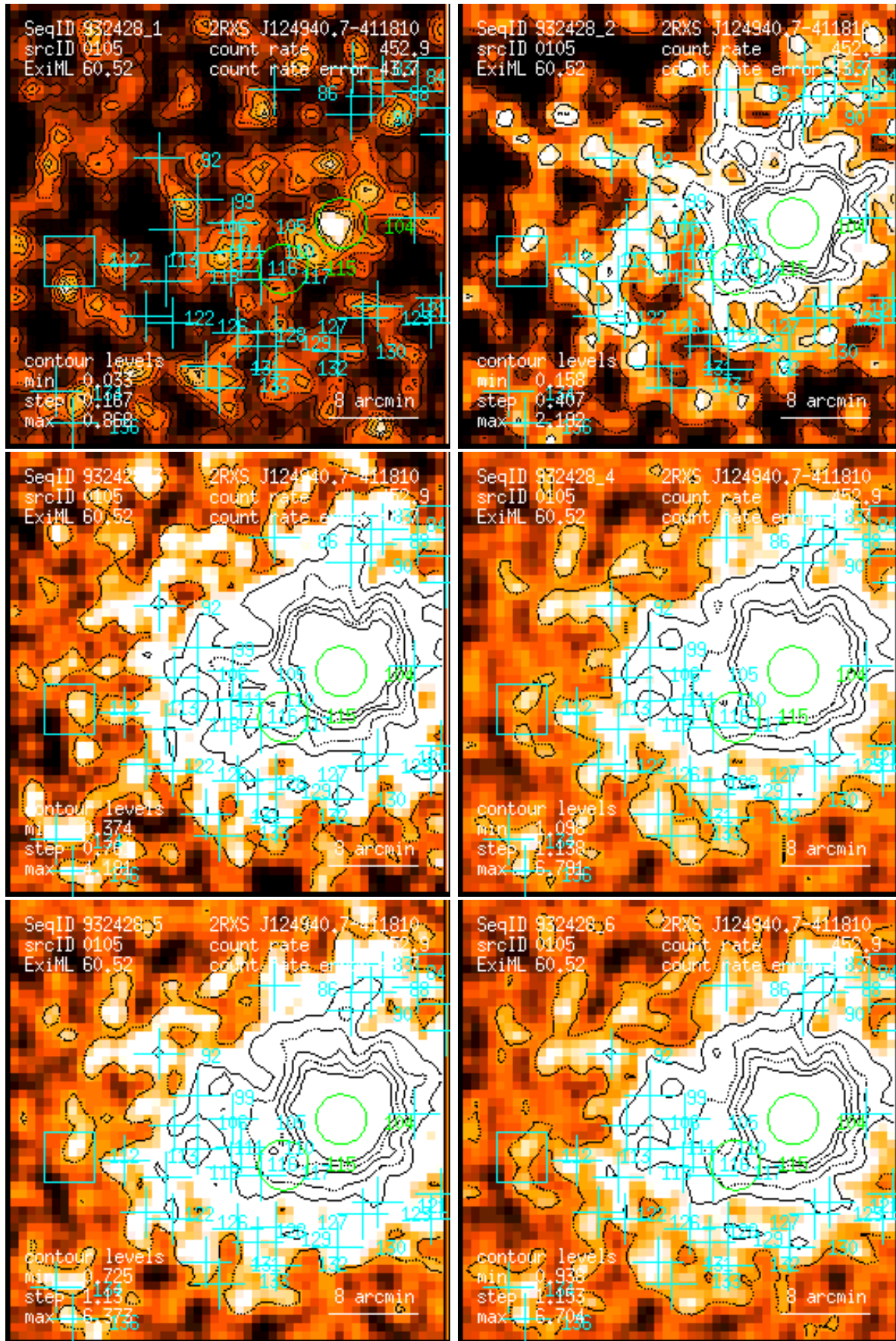
Figure 105: RASS 932428: detection 0105: band rate images, Gaussian filter: (1) PSPC channels 11 – 41, (2) 52 – 90, (3) 91 – 201, (4) 11 – 235, (5) 52 – 201, (6) 11 – 201. Broad band rates in counts/ks. Band rate contour levels in counts/ks/arcmin 2 .
