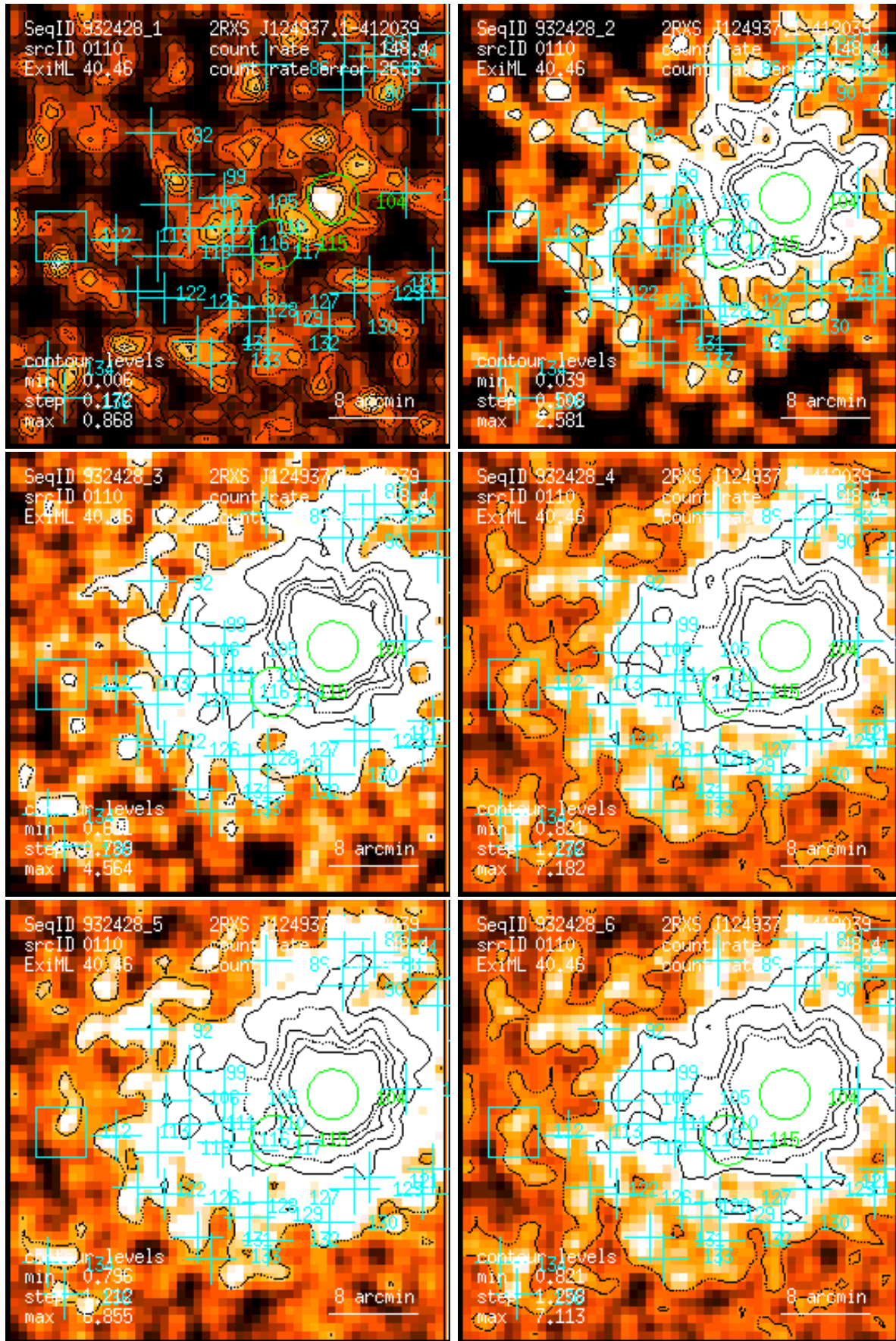
Figure 110: RASS 932428: detection 0110: band rate images, Gaussian filter: (1) PSPC channels 11 – 41, (2) 52 – 90, (3) 91 – 201, (4) 11 – 235, (5) 52 – 201, (6) 11 – 201. Broad band rates in counts/ks. Band rate contour levels in counts/ks/arcmin 2 .
