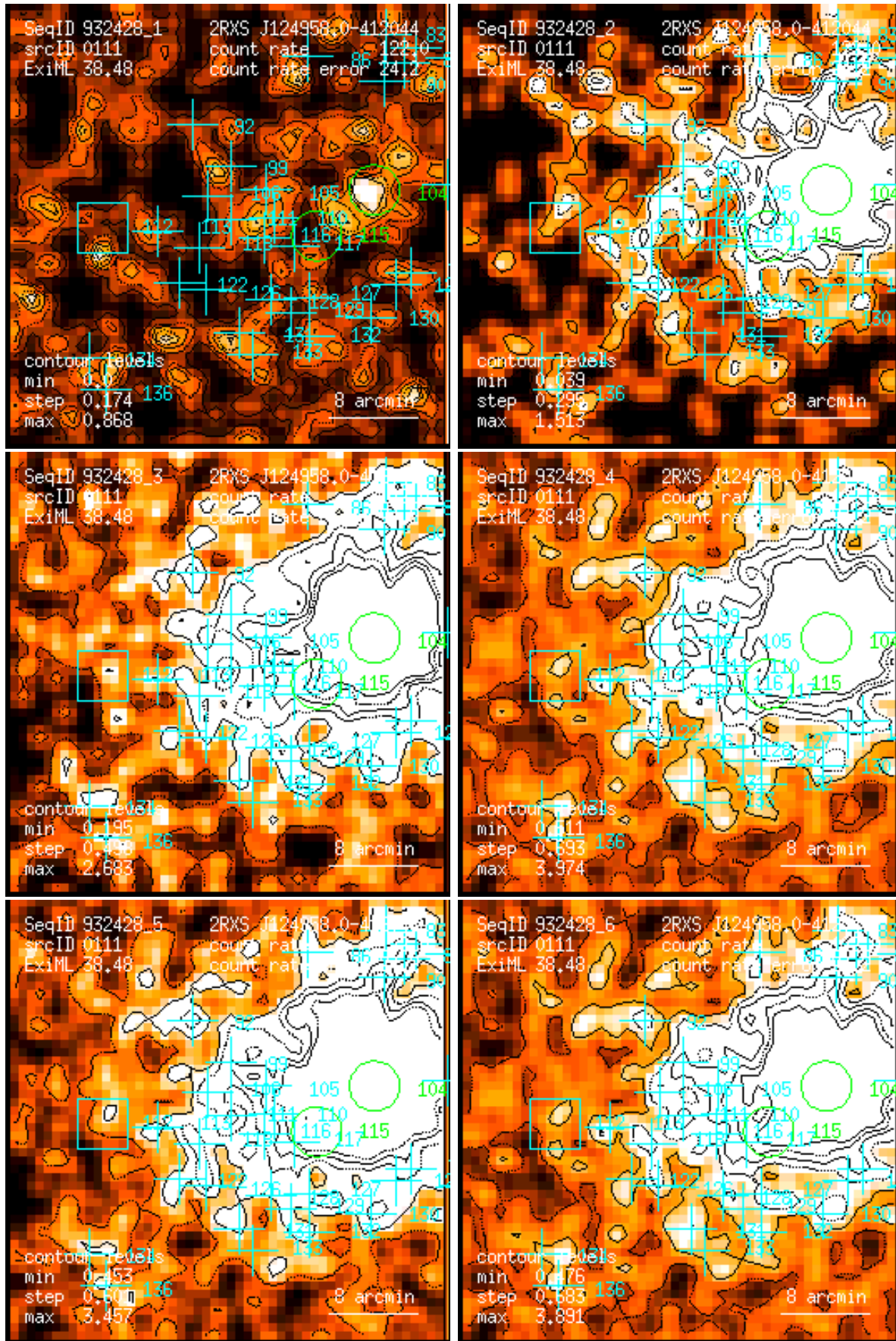
Figure 111: RASS 932428: detection 0111: band rate images, Gaussian filter: (1) PSPC channels 11 – 41, (2) 52 – 90, (3) 91 – 201, (4) 11 – 235, (5) 52 – 201, (6) 11 – 201. Broad band rates in counts/ks. Band rate contour levels in counts/ks/arcmin 2 .
