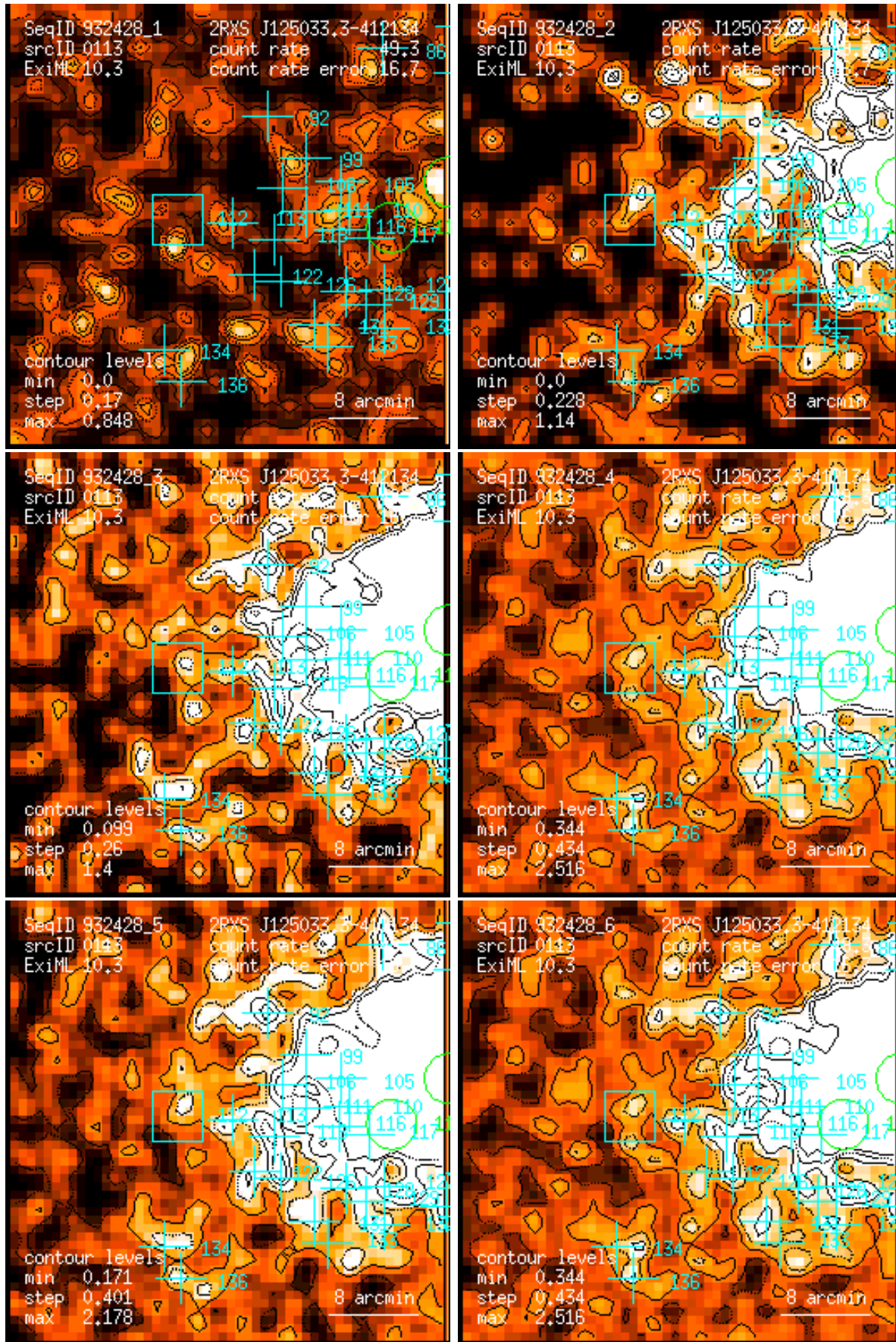
Figure 113: RASS 932428: detection 0113: band rate images, Gaussian filter: (1) PSPC channels 11 – 41, (2) 52 – 90, (3) 91 – 201, (4) 11 – 235, (5) 52 – 201, (6) 11 – 201. Broad band rates in counts/ks. Band rate contour levels in counts/ks/arcmin 2 .
