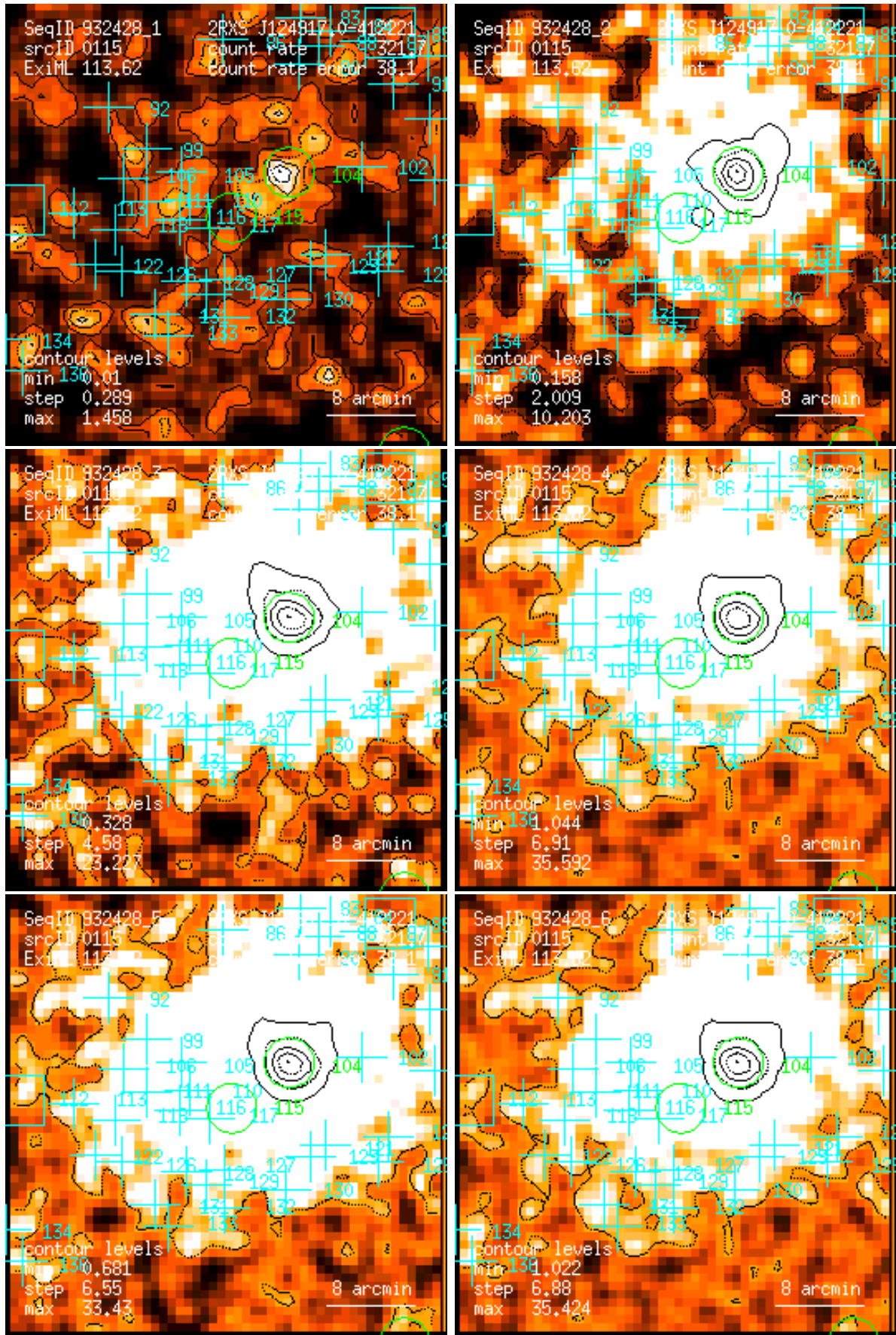
Figure 115: RASS 932428: detection 0115: band rate images, Gaussian filter: (1) PSPC channels 11 – 41, (2) 52 – 90, (3) 91 – 201, (4) 11 – 235, (5) 52 – 201, (6) 11 – 201. Broad band rates in counts/ks. Band rate contour levels in counts/ks/arcmin 2 .
