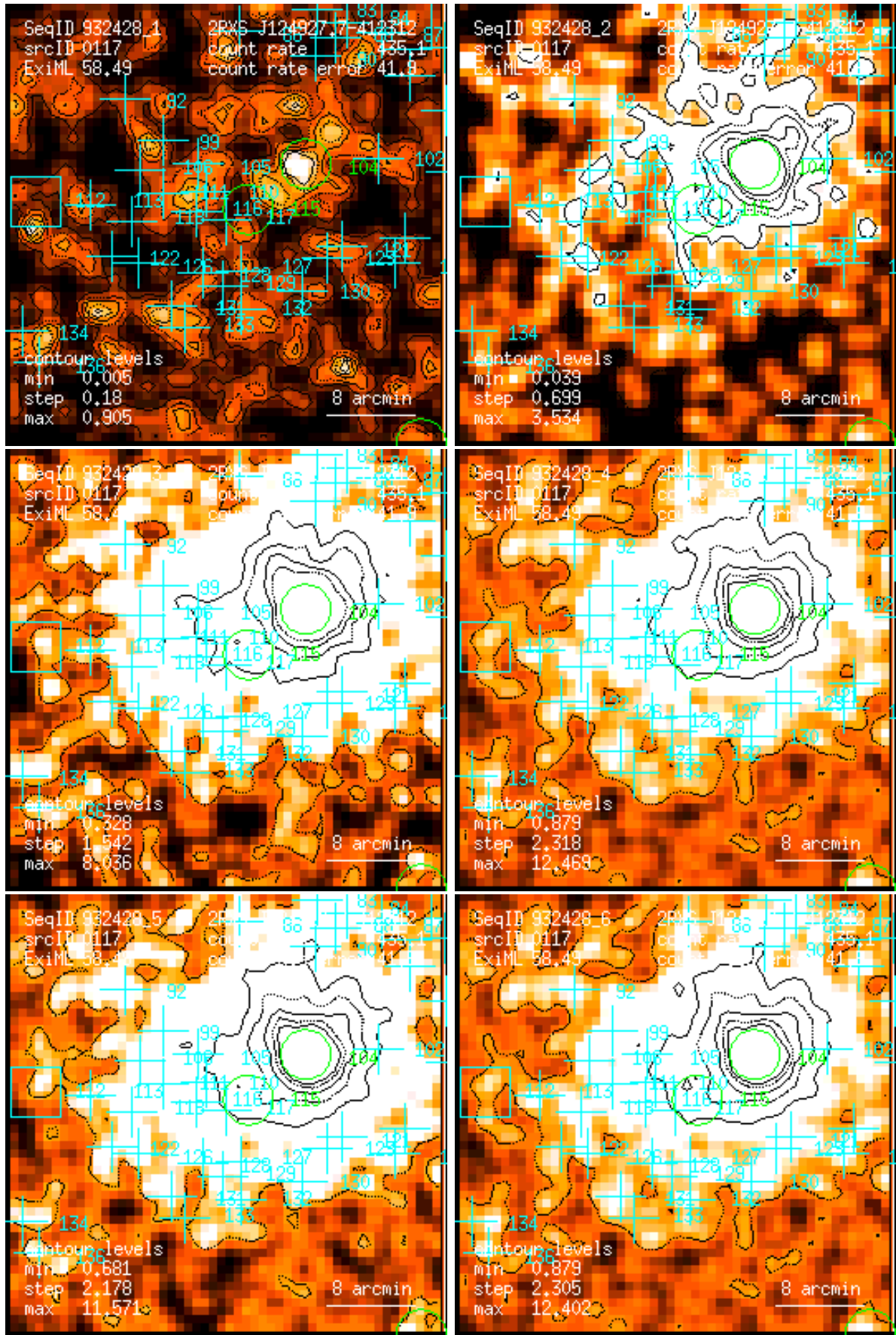
Figure 117: RASS 932428: detection 0117: band rate images, Gaussian filter: (1) PSPC channels 11 – 41, (2) 52 – 90, (3) 91 – 201, (4) 11 – 235, (5) 52 – 201, (6) 11 – 201. Broad band rates in counts/ks. Band rate contour levels in counts/ks/arcmin 2 .
