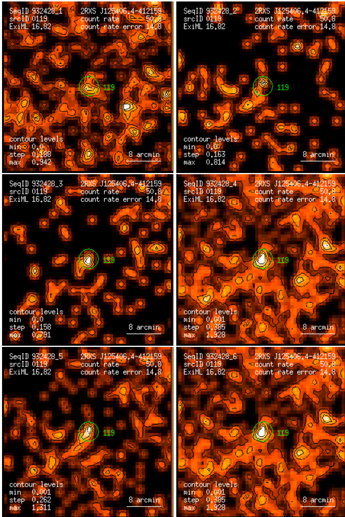
Figure 119: RASS 932428: detection 0119: band rate images, Gaussian filter: (1) PSPC channels 11 – 41, (2) 52 – 90, (3) 91 – 201, (4) 11 – 235, (5) 52 – 201, (6) 11 – 201. Broad band rates in counts/ks. Band rate contour levels in counts/ks/arcmin 2 .
