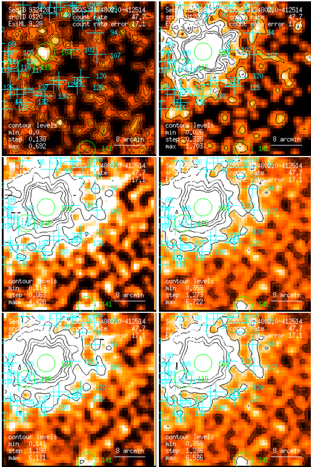
Figure 120: RASS 932428: detection 0120: band rate images, Gaussian filter: (1) PSPC channels 11 – 41, (2) 52 – 90, (3) 91 – 201, (4) 11 – 235, (5) 52 – 201, (6) 11 – 201. Broad band rates in counts/ks. Band rate contour levels in counts/ks/arcmin 2 .
