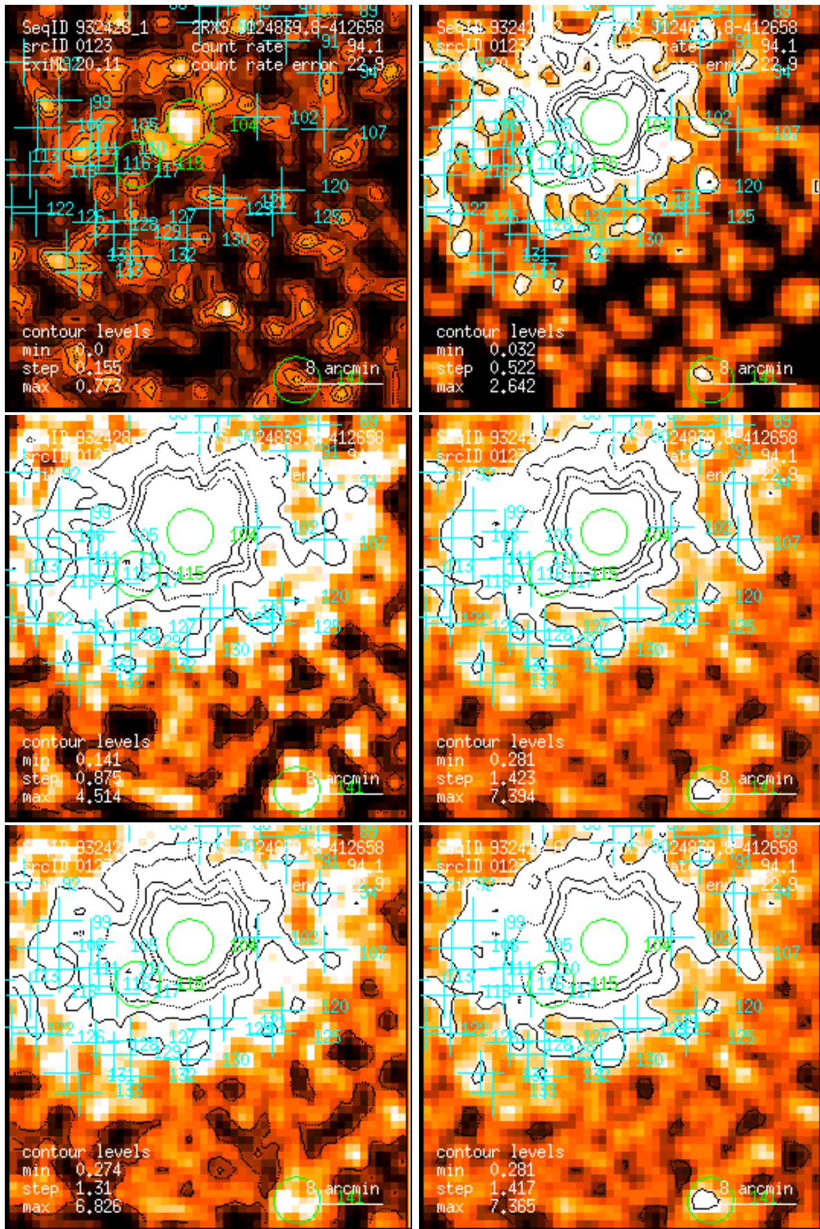
Figure 123: RASS 932428: detection 0123: band rate images, Gaussian filter: (1) PSPC channels 11 – 41, (2) 52 – 90, (3) 91 – 201, (4) 11 – 235, (5) 52 – 201, (6) 11 – 201. Broad band rates in counts/ks. Band rate contour levels in counts/ks/arcmin 2 .
