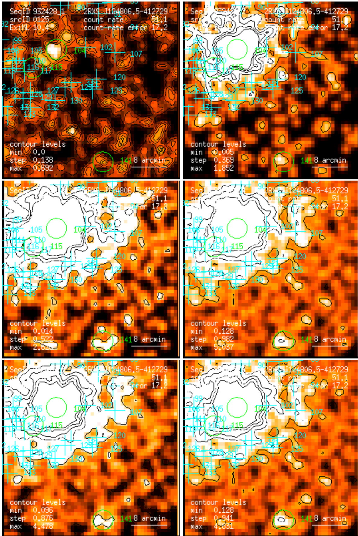
Figure 125: RASS 932428: detection 0125: band rate images, Gaussian filter: (1) PSPC channels 11 – 41, (2) 52 – 90, (3) 91 – 201, (4) 11 – 235, (5) 52 – 201, (6) 11 – 201. Broad band rates in counts/ks. Band rate contour levels in counts/ks/arcmin 2 .
