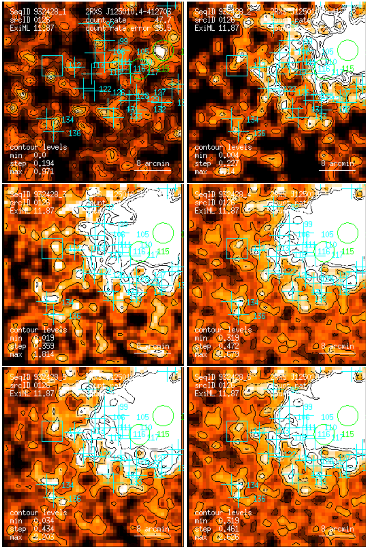
Figure 126: RASS 932428: detection 0126: band rate images, Gaussian filter: (1) PSPC channels 11 – 41, (2) 52 – 90, (3) 91 – 201, (4) 11 – 235, (5) 52 – 201, (6) 11 – 201. Broad band rates in counts/ks. Band rate contour levels in counts/ks/arcmin 2 .
