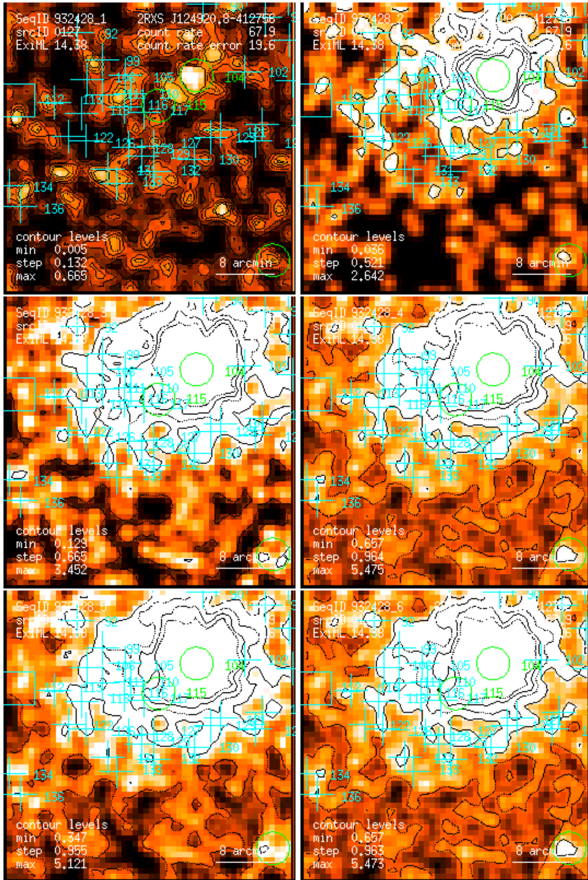
Figure 127: RASS 932428: detection 0127: band rate images, Gaussian filter: (1) PSPC channels 11 – 41, (2) 52 – 90, (3) 91 – 201, (4) 11 – 235, (5) 52 – 201, (6) 11 – 201. Broad band rates in counts/ks. Band rate contour levels in counts/ks/arcmin 2 .
