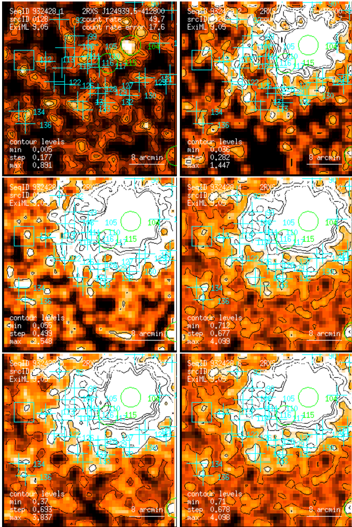
Figure 128: RASS 932428: detection 0128: band rate images, Gaussian filter: (1) PSPC channels 11 – 41, (2) 52 – 90, (3) 91 – 201, (4) 11 – 235, (5) 52 – 201, (6) 11 – 201. Broad band rates in counts/ks. Band rate contour levels in counts/ks/arcmin 2 .
