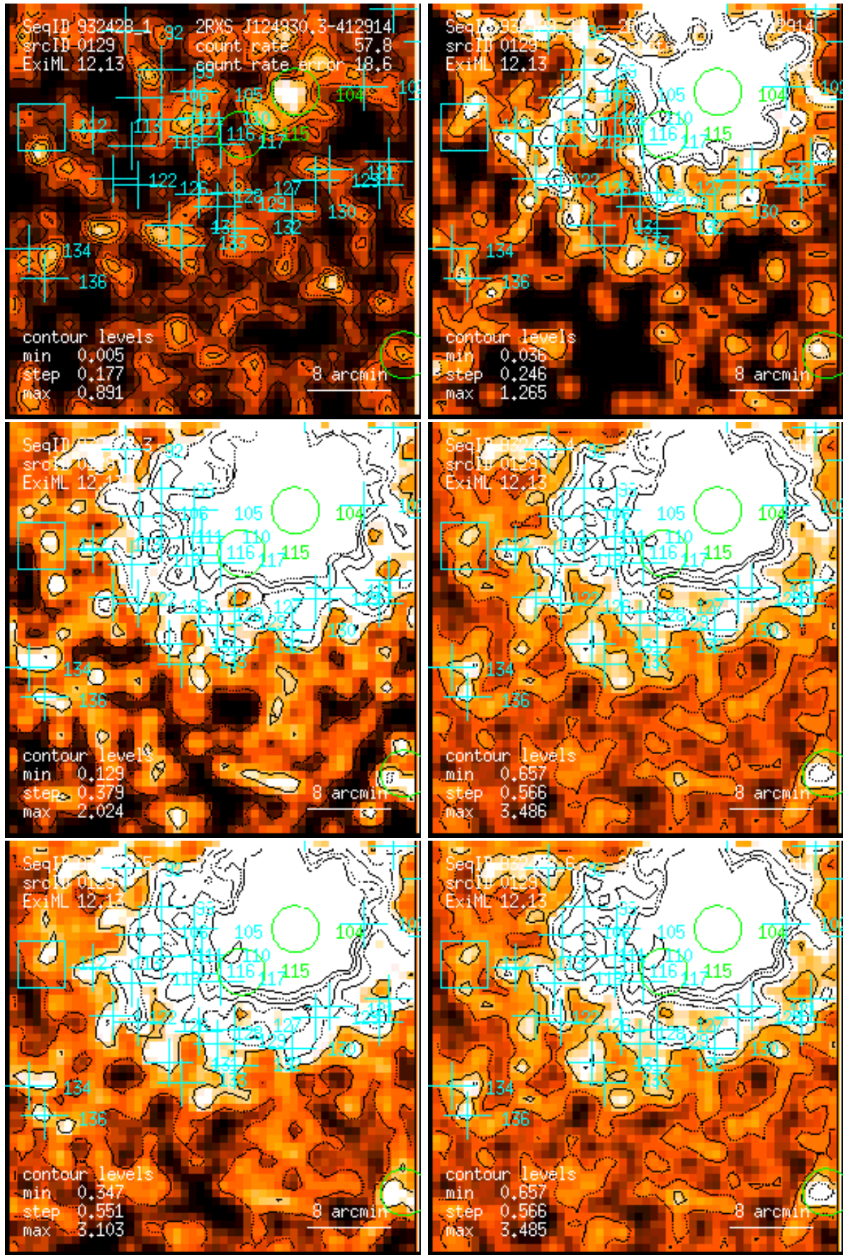
Figure 129: RASS 932428: detection 0129: band rate images, Gaussian filter: (1) PSPC channels 11 – 41, (2) 52 – 90, (3) 91 – 201, (4) 11 – 235, (5) 52 – 201, (6) 11 – 201. Broad band rates in counts/ks. Band rate contour levels in counts/ks/arcmin 2 .
