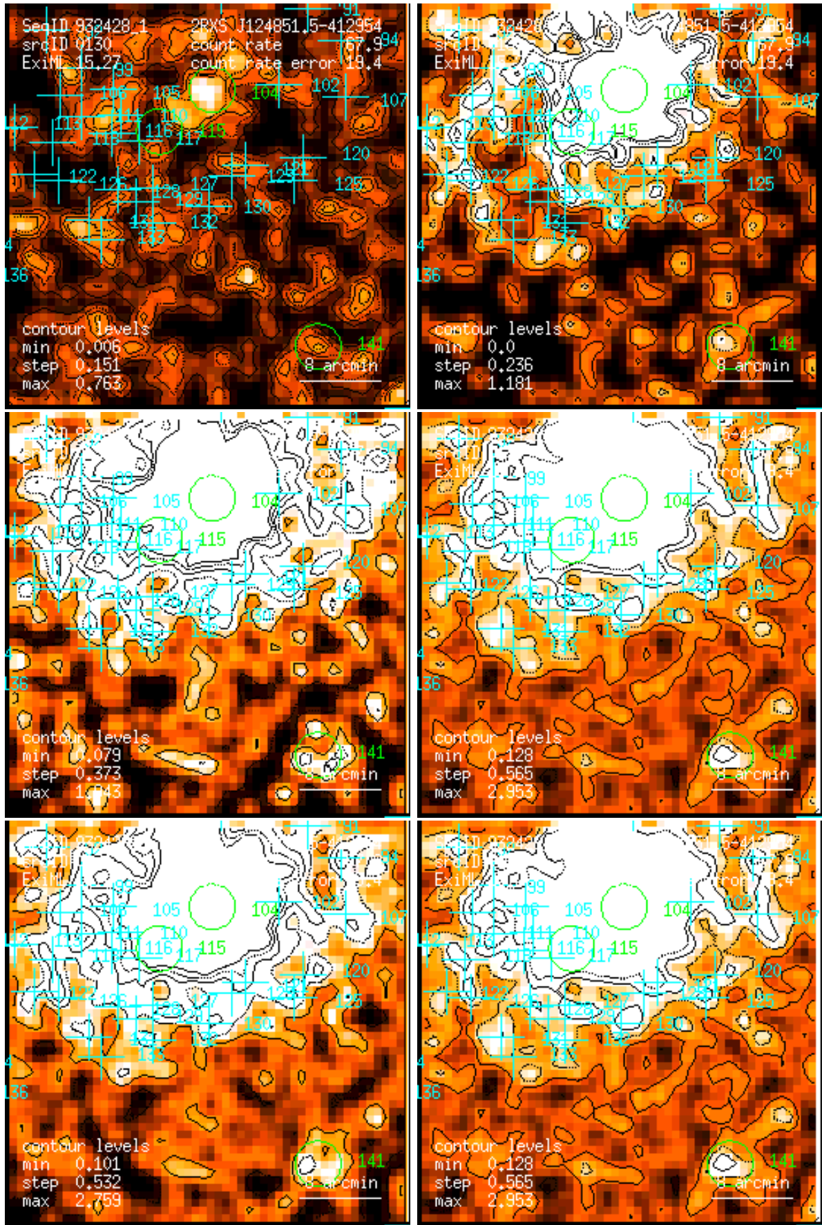
Figure 130: RASS 932428: detection 0130: band rate images, Gaussian filter: (1) PSPC channels 11 – 41, (2) 52 – 90, (3) 91 – 201, (4) 11 – 235, (5) 52 – 201, (6) 11 – 201. Broad band rates in counts/ks. Band rate contour levels in counts/ks/arcmin 2 .
