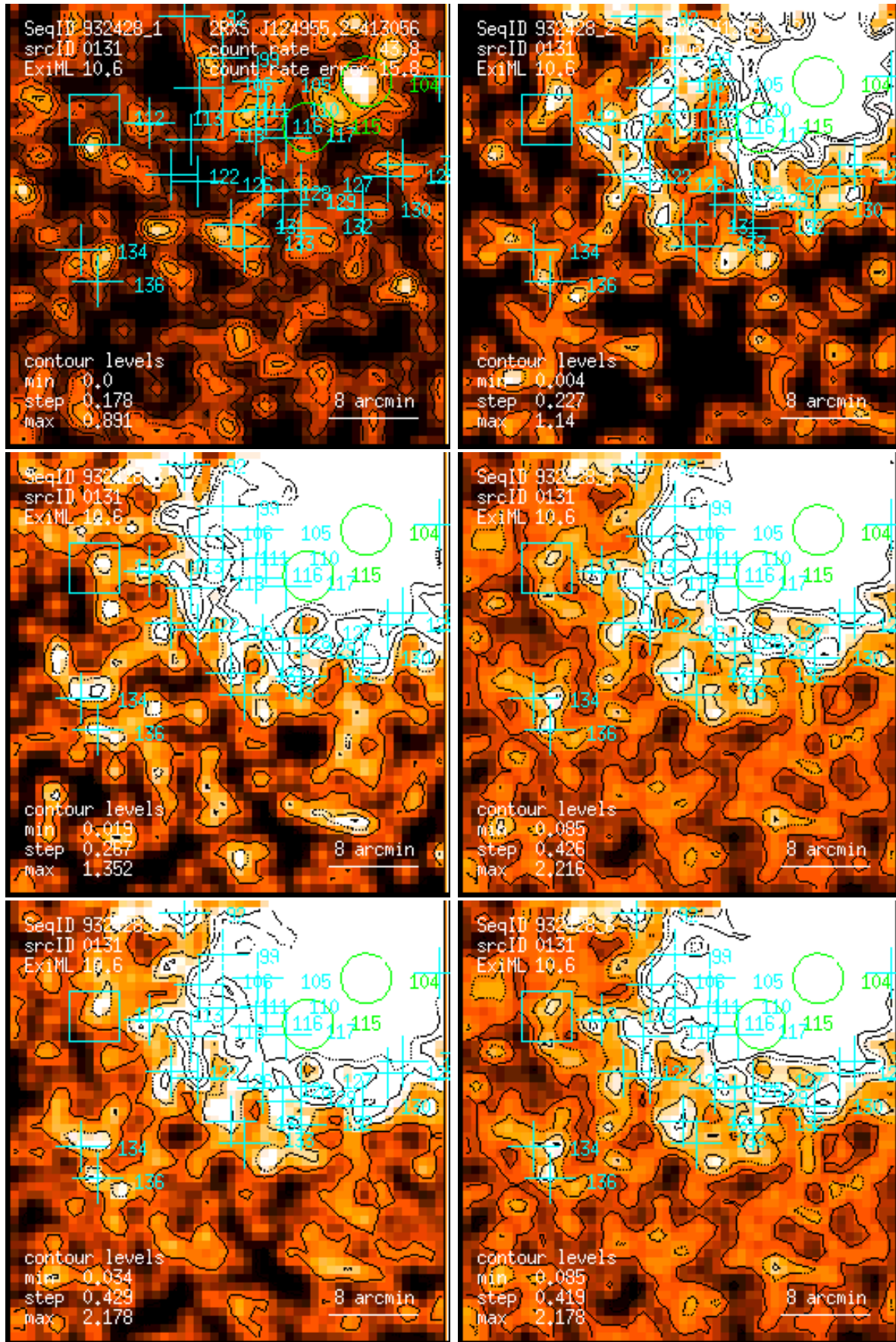
Figure 131: RASS 932428: detection 0131: band rate images, Gaussian filter: (1) PSPC channels 11 – 41, (2) 52 – 90, (3) 91 – 201, (4) 11 – 235, (5) 52 – 201, (6) 11 – 201. Broad band rates in counts/ks. Band rate contour levels in counts/ks/arcmin 2 .
