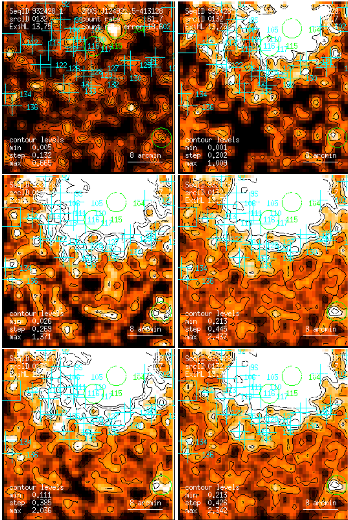
Figure 132: RASS 932428: detection 0132: band rate images, Gaussian filter: (1) PSPC channels 11 – 41, (2) 52 – 90, (3) 91 – 201, (4) 11 – 235, (5) 52 – 201, (6) 11 – 201. Broad band rates in counts/ks. Band rate contour levels in counts/ks/arcmin 2 .
