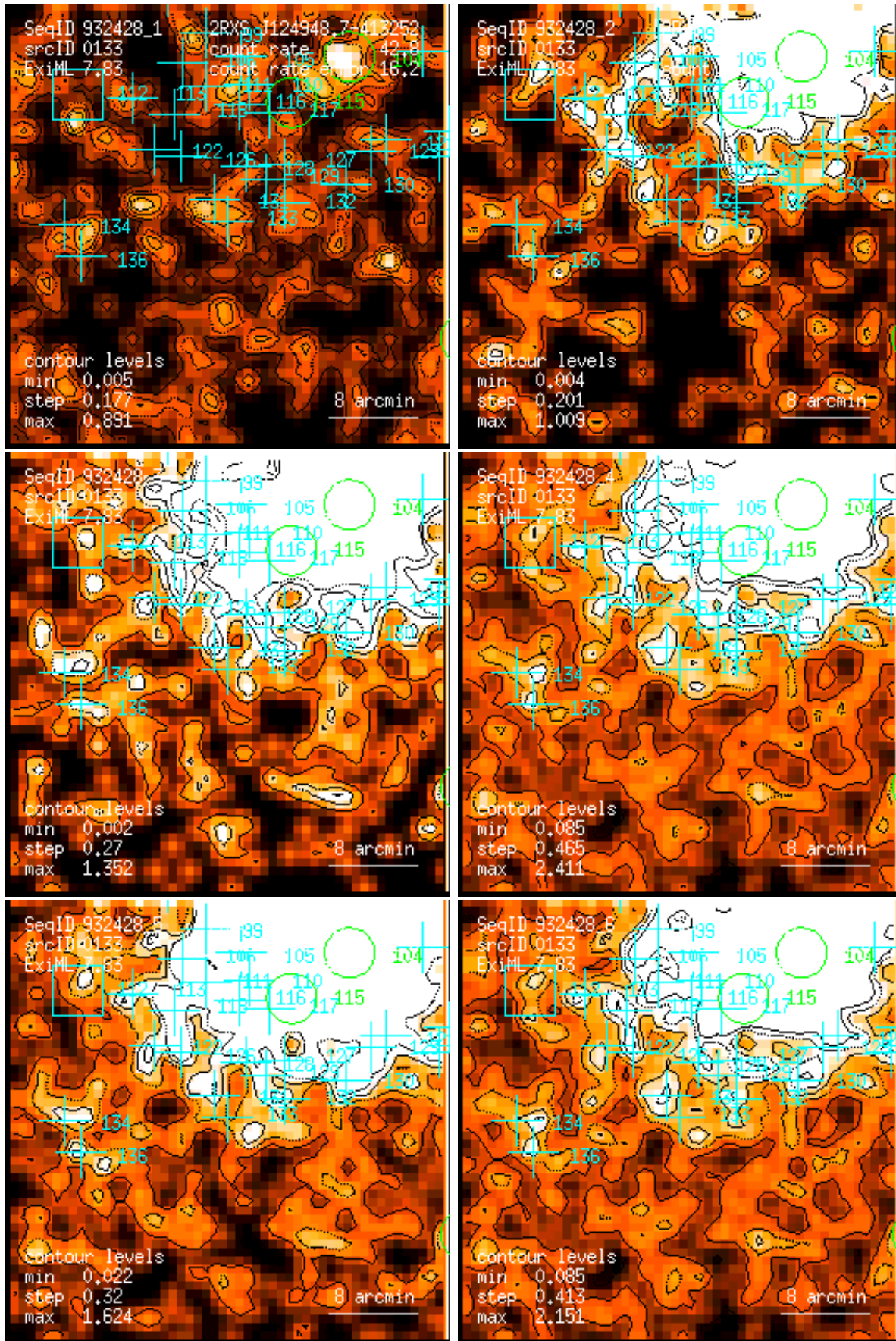
Figure 133: RASS 932428: detection 0133: band rate images, Gaussian filter: (1) PSPC channels 11 – 41, (2) 52 – 90, (3) 91 – 201, (4) 11 – 235, (5) 52 – 201, (6) 11 – 201. Broad band rates in counts/ks. Band rate contour levels in counts/ks/arcmin 2 .
