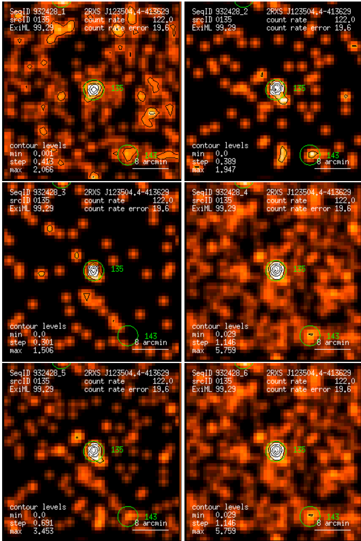
Figure 135: RASS 932428: detection 0135: band rate images, Gaussian filter: (1) PSPC channels 11 – 41, (2) 52 – 90, (3) 91 – 201, (4) 11 – 235, (5) 52 – 201, (6) 11 – 201. Broad band rates in counts/ks. Band rate contour levels in counts/ks/arcmin 2 .
