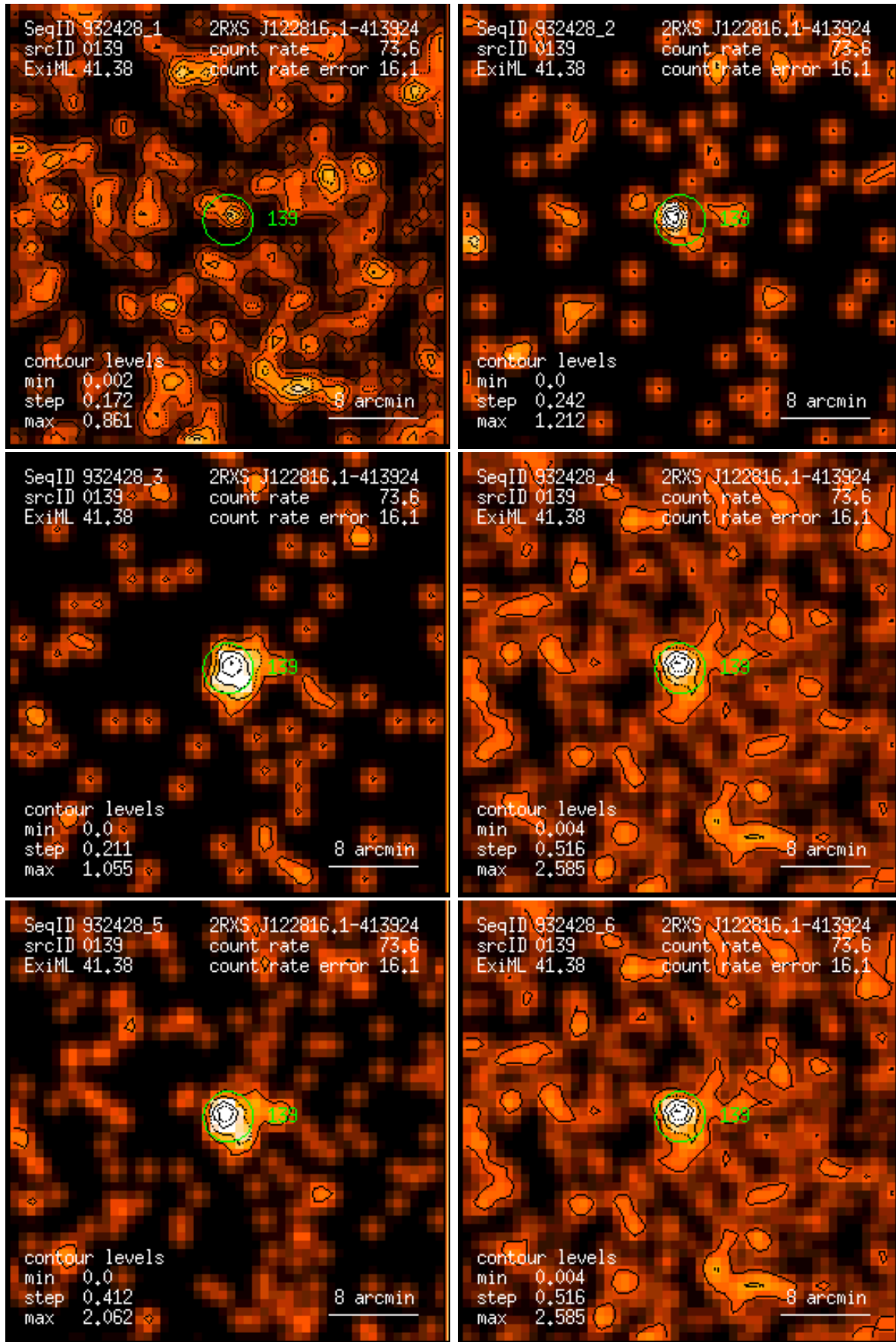
Figure 139: RASS 932428: detection 0139: band rate images, Gaussian filter: (1) PSPC channels 11 – 41, (2) 52 – 90, (3) 91 – 201, (4) 11 – 235, (5) 52 – 201, (6) 11 – 201. Broad band rates in counts/ks. Band rate contour levels in counts/ks/arcmin 2 .
