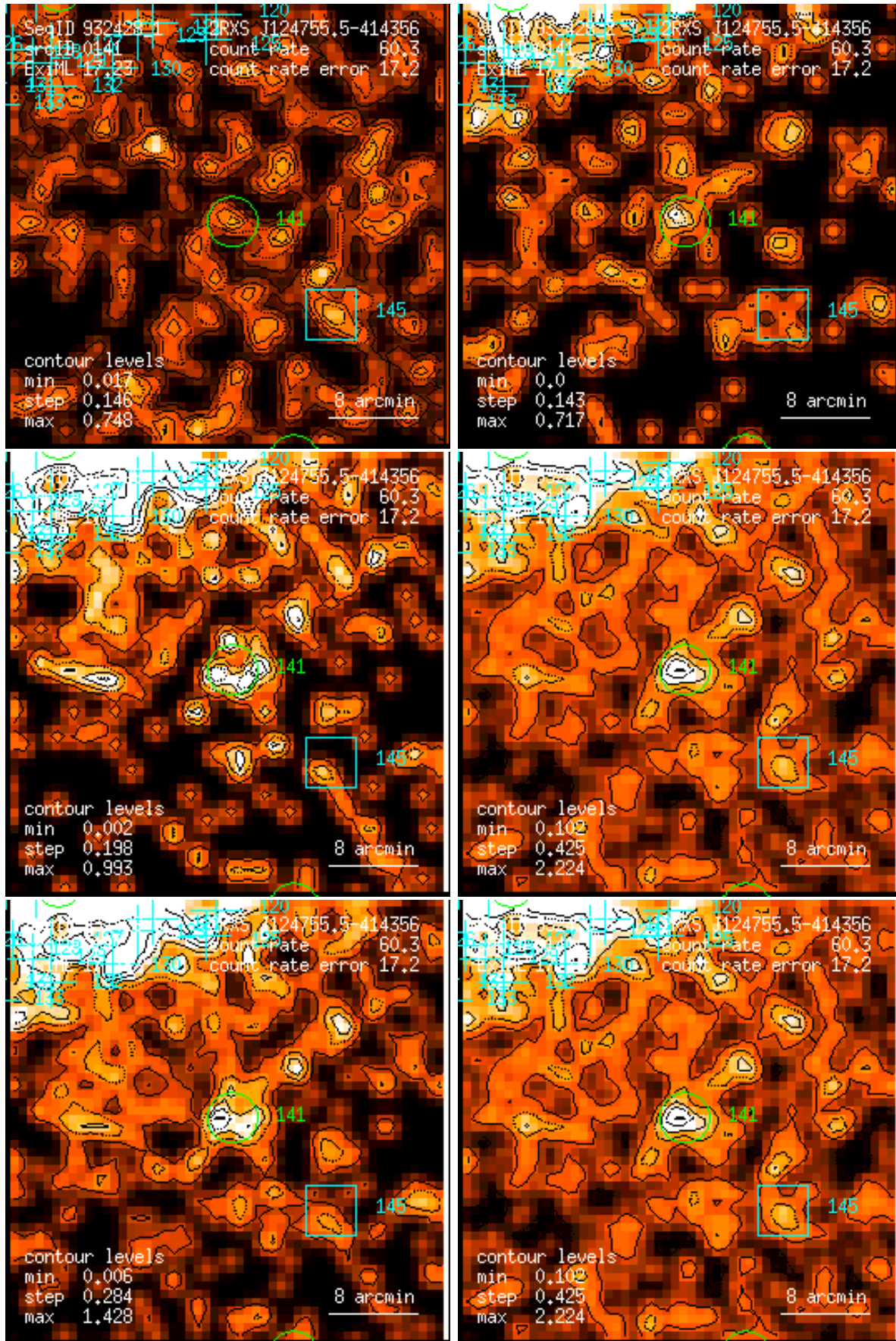
Figure 141: RASS 932428: detection 0141: band rate images, Gaussian filter: (1) PSPC channels 11 – 41, (2) 52 – 90, (3) 91 – 201, (4) 11 – 235, (5) 52 – 201, (6) 11 – 201. Broad band rates in counts/ks. Band rate contour levels in counts/ks/arcmin 2 .
