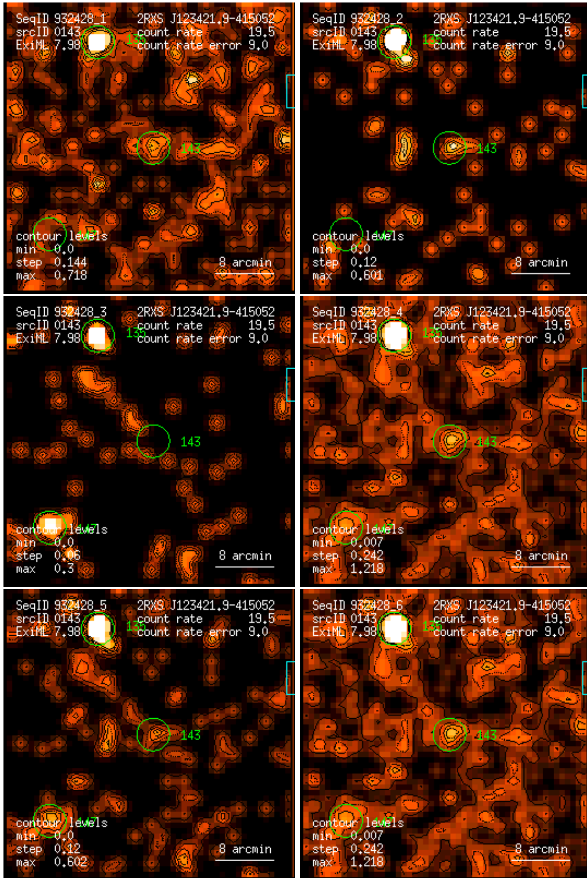
Figure 143: RASS 932428: detection 0143: band rate images, Gaussian filter: (1) PSPC channels 11 – 41, (2) 52 – 90, (3) 91 – 201, (4) 11 – 235, (5) 52 – 201, (6) 11 – 201. Broad band rates in counts/ks. Band rate contour levels in counts/ks/arcmin 2 .
