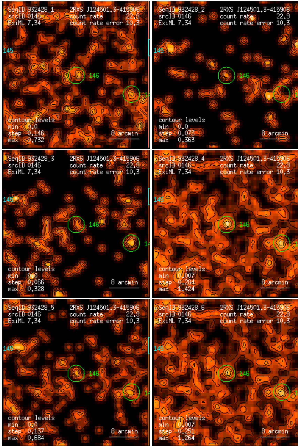
Figure 146: RASS 932428: detection 0146: band rate images, Gaussian filter: (1) PSPC channels 11 – 41, (2) 52 – 90, (3) 91 – 201, (4) 11 – 235, (5) 52 – 201, (6) 11 – 201. Broad band rates in counts/ks. Band rate contour levels in counts/ks/arcmin 2 .
