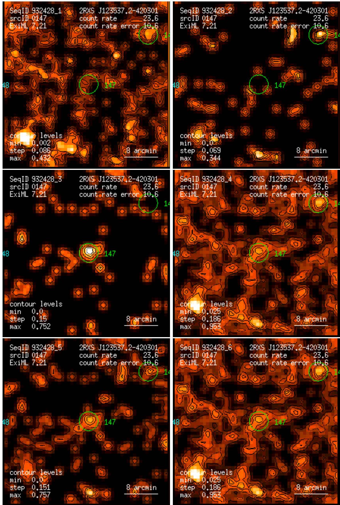
Figure 147: RASS 932428: detection 0147: band rate images, Gaussian filter: (1) PSPC channels 11 – 41, (2) 52 – 90, (3) 91 – 201, (4) 11 – 235, (5) 52 – 201, (6) 11 – 201. Broad band rates in counts/ks. Band rate contour levels in counts/ks/arcmin 2 .
