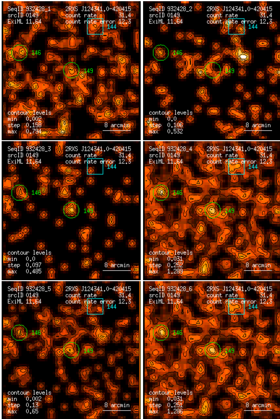
Figure 149: RASS 932428: detection 0149: band rate images, Gaussian filter: (1) PSPC channels 11 – 41, (2) 52 – 90, (3) 91 – 201, (4) 11 – 235, (5) 52 – 201, (6) 11 – 201. Broad band rates in counts/ks. Band rate contour levels in counts/ks/arcmin 2 .
