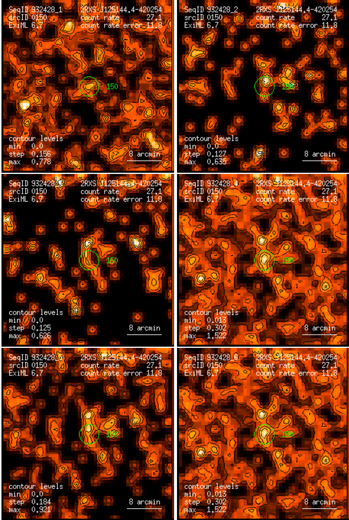
Figure 150: RASS 932428: detection 0150: band rate images, Gaussian filter: (1) PSPC channels 11 – 41, (2) 52 – 90, (3) 91 – 201, (4) 11 – 235, (5) 52 – 201, (6) 11 – 201. Broad band rates in counts/ks. Band rate contour levels in counts/ks/arcmin 2 .
