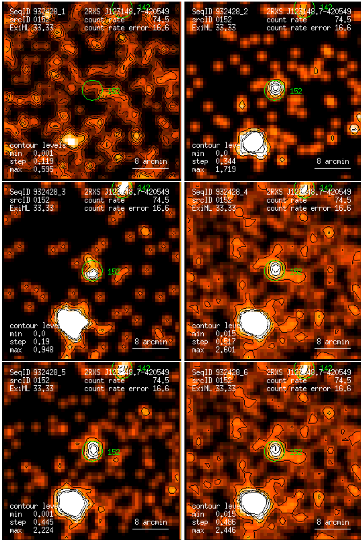
Figure 152: RASS 932428: detection 0152: band rate images, Gaussian filter: (1) PSPC channels 11 – 41, (2) 52 – 90, (3) 91 – 201, (4) 11 – 235, (5) 52 – 201, (6) 11 – 201. Broad band rates in counts/ks. Band rate contour levels in counts/ks/arcmin 2 .
