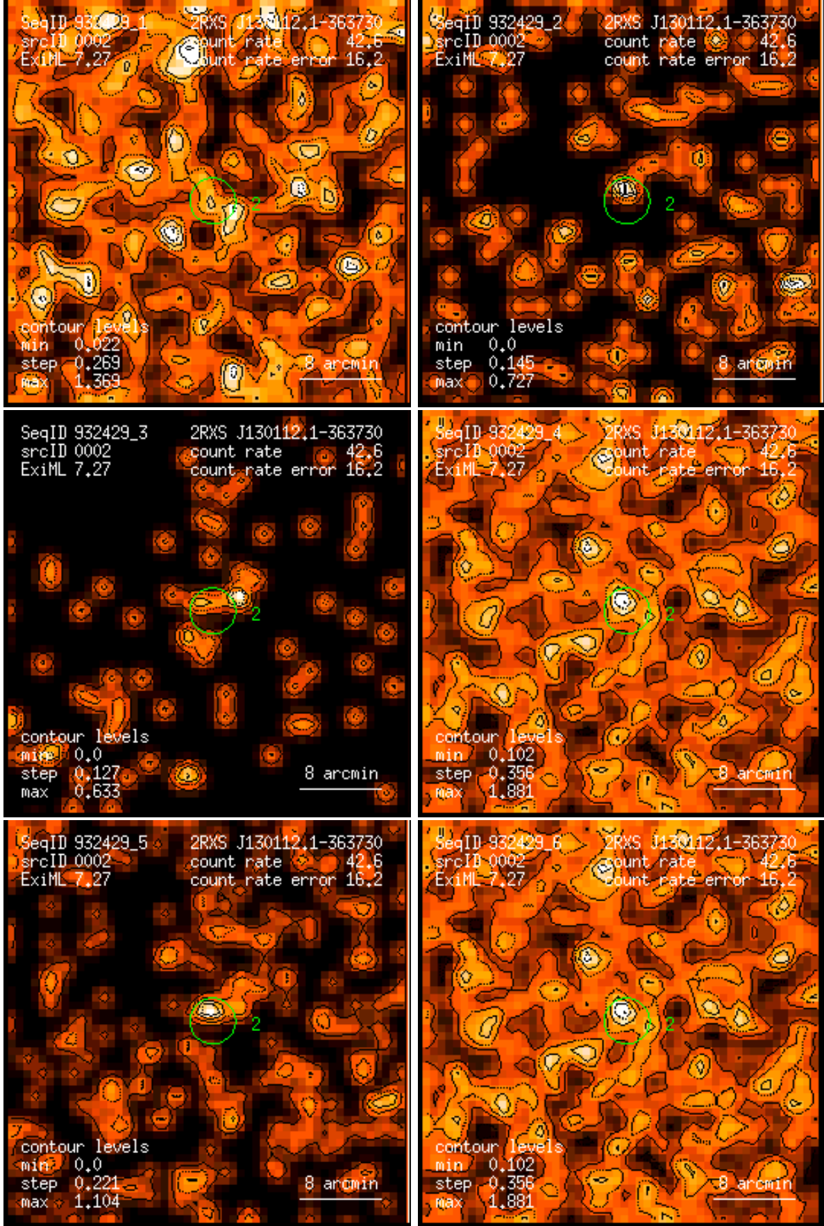
Figure 2: RASS 932429: detection 0002: band rate images, Gaussian filter: (1) PSPC channels 11 – 41, (2) 52 – 90, (3) 91 – 201, (4) 11 – 235, (5) 52 – 201, (6) 11 – 201. Broad band rates in counts/ks. Band rate contour levels in counts/ks/arcmin 2 .
