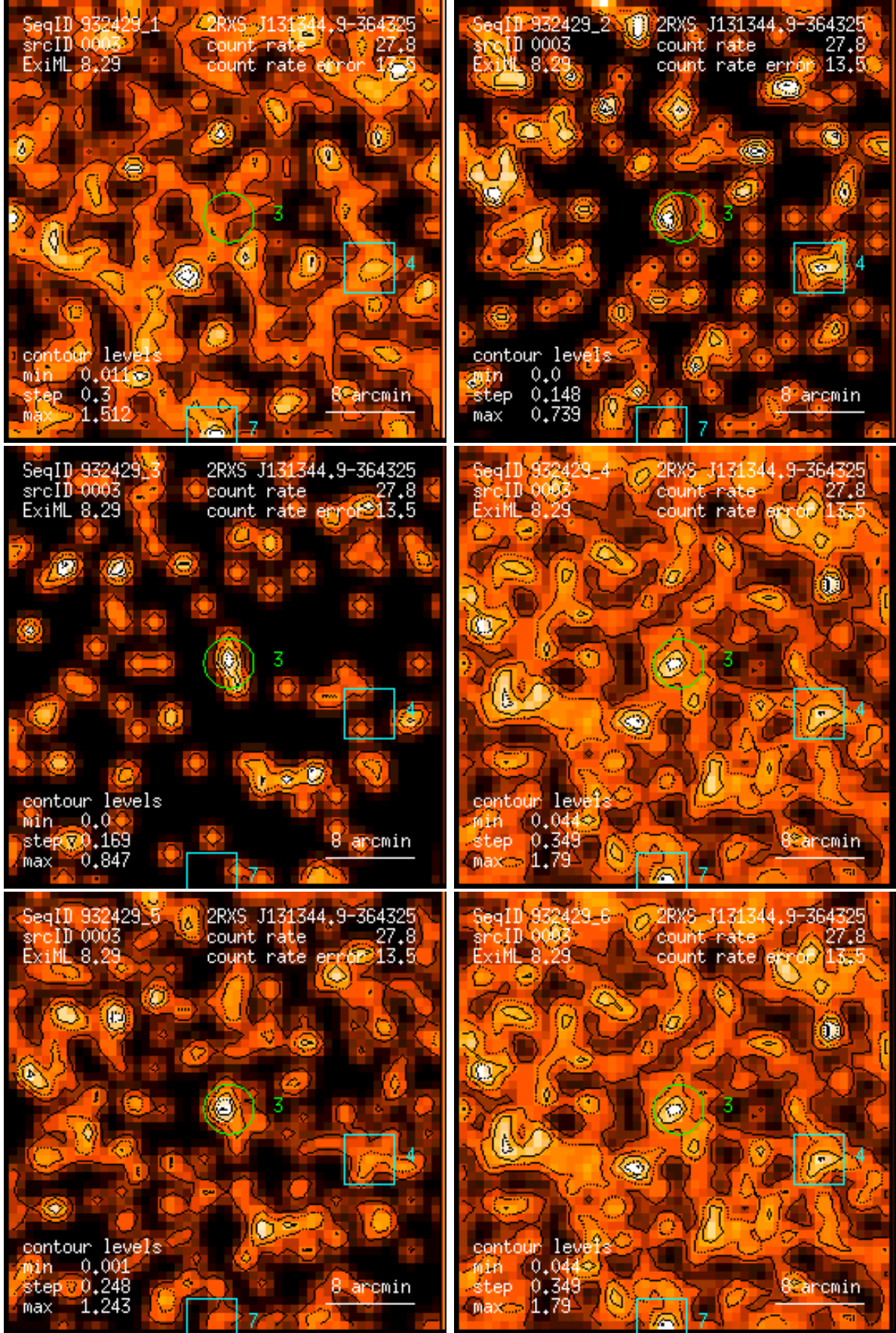
Figure 3: RASS 932429: detection 0003: band rate images, Gaussian filter: (1) PSPC channels 11 – 41, (2) 52 – 90, (3) 91 – 201, (4) 11 – 235, (5) 52 – 201, (6) 11 – 201. Broad band rates in counts/ks. Band rate contour levels in counts/ks/arcmin 2 .
