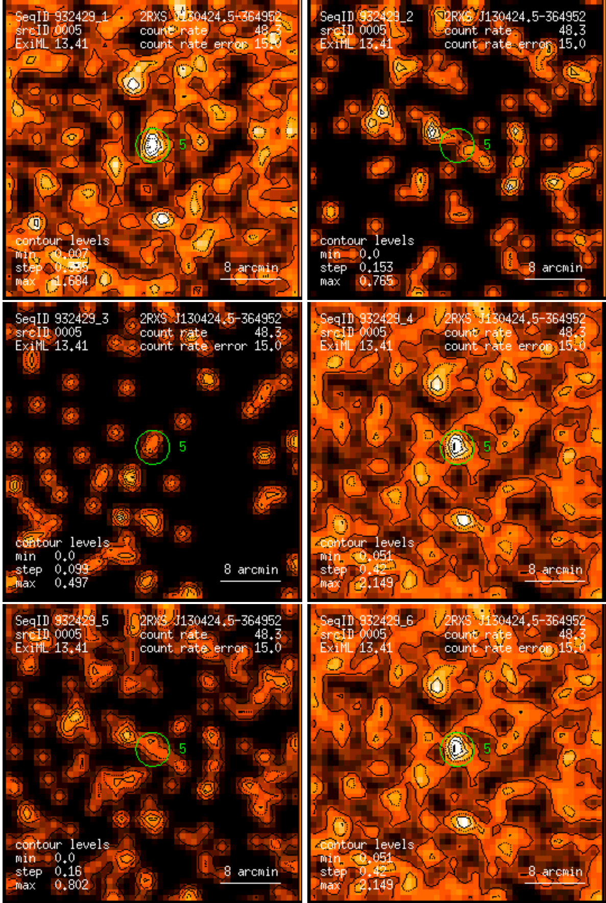
Figure 5: RASS 932429: detection 0005: band rate images, Gaussian filter: (1) PSPC channels 11 – 41, (2) 52 – 90, (3) 91 – 201, (4) 11 – 235, (5) 52 – 201, (6) 11 – 201. Broad band rates in counts/ks. Band rate contour levels in counts/ks/arcmin 2 .
