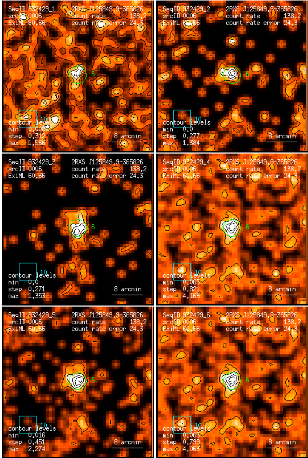
Figure 6: RASS 932429: detection 0006: band rate images, Gaussian filter: (1) PSPC channels 11 – 41, (2) 52 – 90, (3) 91 – 201, (4) 11 – 235, (5) 52 – 201, (6) 11 – 201. Broad band rates in counts/ks. Band rate contour levels in counts/ks/arcmin 2 .
