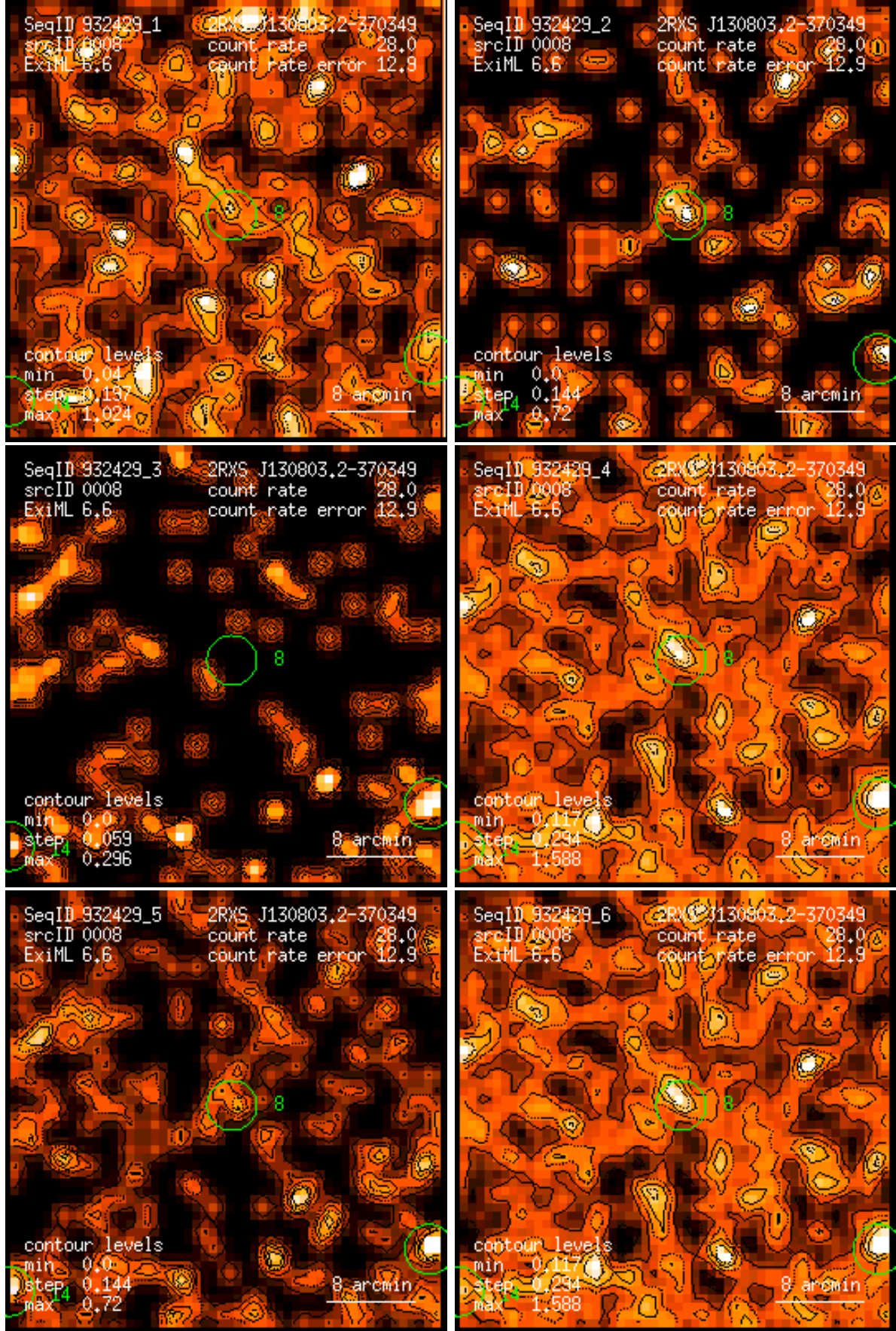
Figure 8: RASS 932429: detection 0008: band rate images, Gaussian filter: (1) PSPC channels 11 – 41, (2) 52 – 90, (3) 91 – 201, (4) 11 – 235, (5) 52 – 201, (6) 11 – 201. Broad band rates in counts/ks. Band rate contour levels in counts/ks/arcmin 2 .
