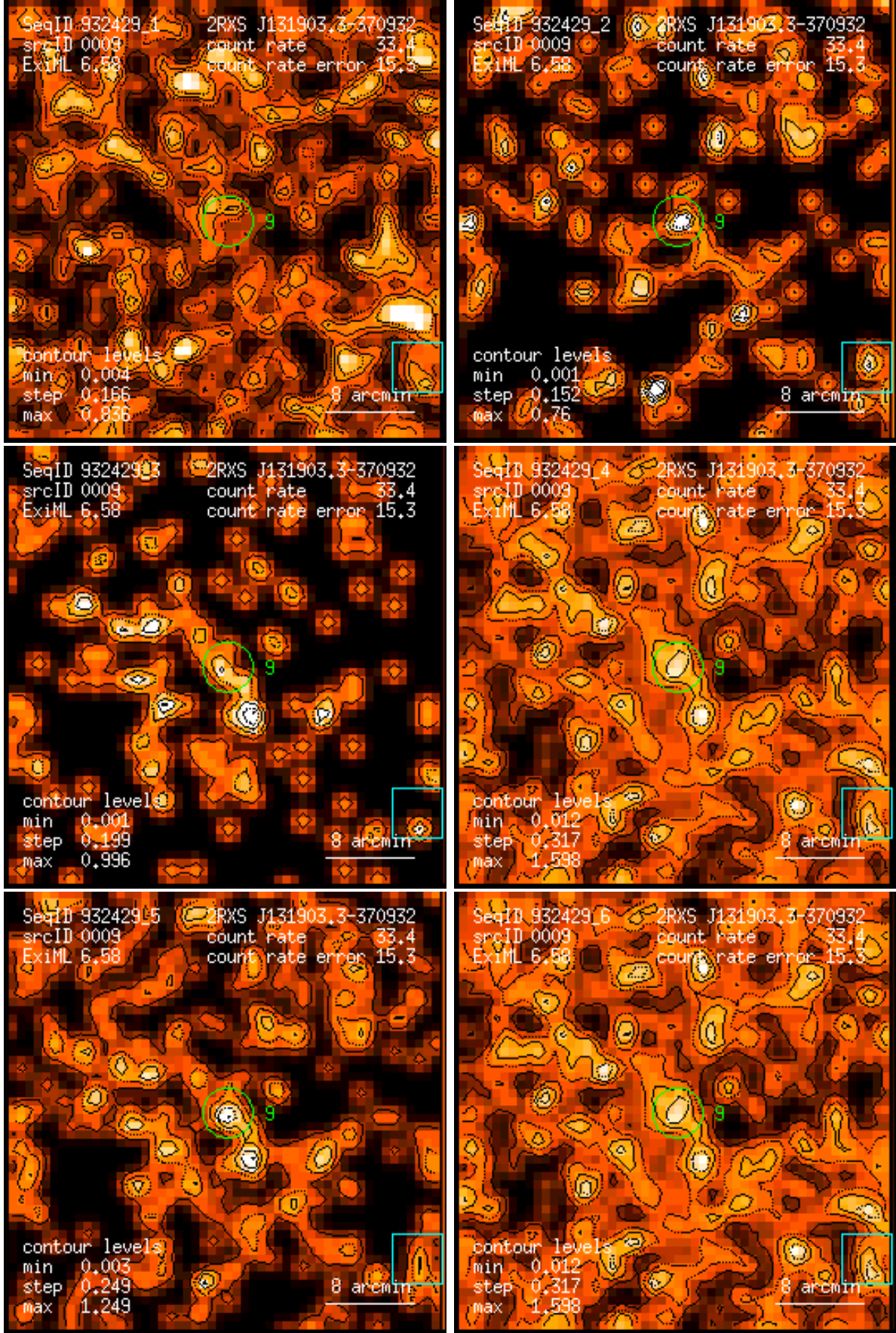
Figure 9: RASS 932429: detection 0009: band rate images, Gaussian filter: (1) PSPC channels 11 – 41, (2) 52 – 90, (3) 91 – 201, (4) 11 – 235, (5) 52 – 201, (6) 11 – 201. Broad band rates in counts/ks. Band rate contour levels in counts/ks/arcmin 2 .
