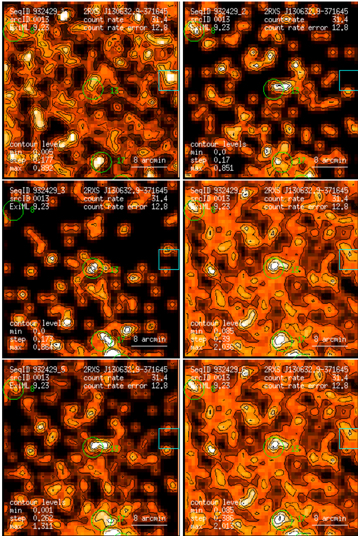
Figure 13: RASS 932429: detection 0013: band rate images, Gaussian filter: (1) PSPC channels 11 – 41, (2) 52 – 90, (3) 91 – 201, (4) 11 – 235, (5) 52 – 201, (6) 11 – 201. Broad band rates in counts/ks. Band rate contour levels in counts/ks/arcmin 2 .
