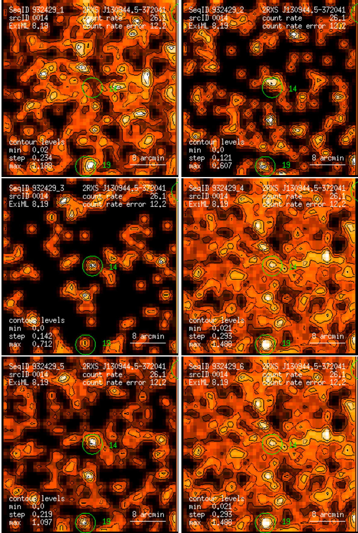
Figure 14: RASS 932429: detection 0014: band rate images, Gaussian filter: (1) PSPC channels 11 – 41, (2) 52 – 90, (3) 91 – 201, (4) 11 – 235, (5) 52 – 201, (6) 11 – 201. Broad band rates in counts/ks. Band rate contour levels in counts/ks/arcmin 2 .
